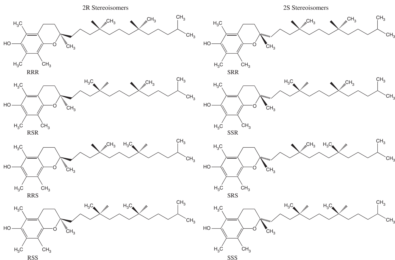
Figure 2 Diagrammatic representation of various stereoisomers of \alpha -tocopherol.
