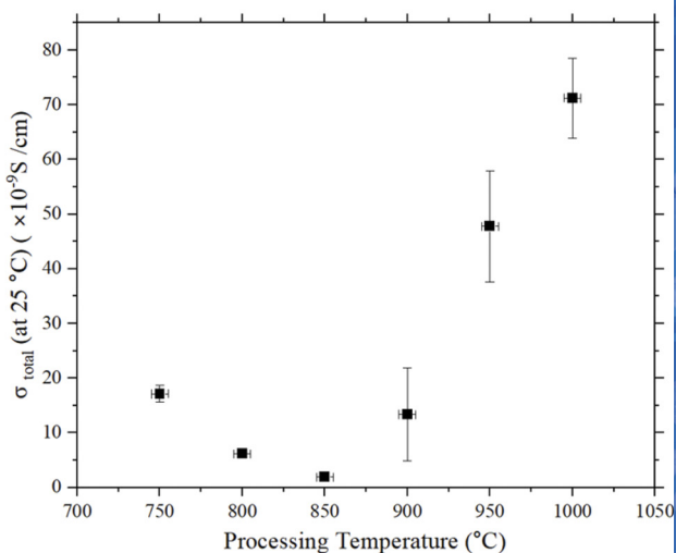
Total Conductivity vs Processing Temperature
