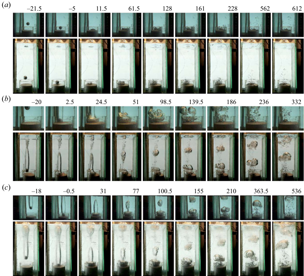
Figure 5. Impact dynamics of the projectile ( D_p = 40 mm) on the granular bed submerged in water for (a) E_k = 1.3 J ( \ell_B^{max} = 0 ), (b) E_k = 3.3 J (pinch-off of the air bubble in the bulk liquid; 0 < \ell_B^{max} < L_W ) and (c) E_k = 4.6 J (surface pinch-off at \partial A ; \ell_B^{max} \approx O(L_W) ). In each panel, the top image depicts the dynamics at the bed, and the bottom shows the dynamics over the entire liquid column captured using different cameras. The time, t in milliseconds (ms), is shown at the top of each panel, with t = 0 ms representing the instant when the projectile touches the granular bed surface.
