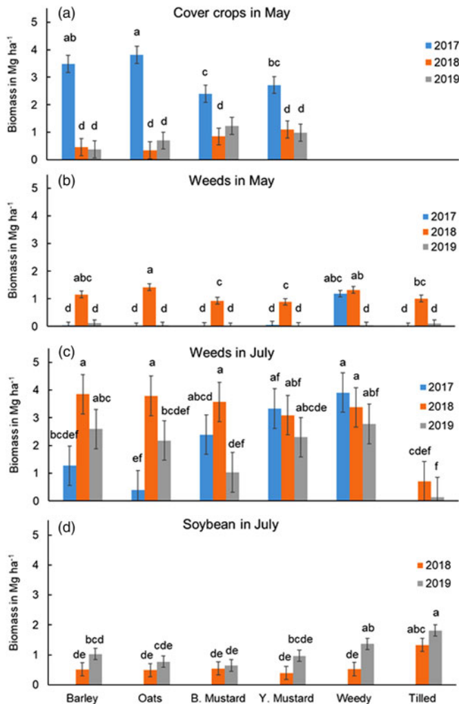
Fig. 1. Biomass of cover crops (CC) at termination (a), weeds at CC termination (b), weed biomass in soybean six weeks after planting (c) and soybean biomass six weeks after planting (d). Treatments were barley CC (Barley), oats CC (Oats), brown mustard CC (B. mustard), yellow mustard CC (Y. mustard), no-CC plots that were not tilled (Weedy) and no-CC plots that were tilled for weed control (Tilled). The study years were 2017 (blue bars), 2018 (red bars), and 2019 (grey bars). Soybean biomass was not available in 2017. Lines above bars indicate standard errors. Bars with the same letters indicate means that are not significantly different from each other at \alpha = 0.05 .
