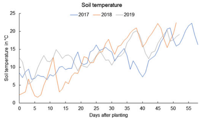
Fig. 2. Soil temperature from the day of CC planting to the day of CC termination for each year of the study.
