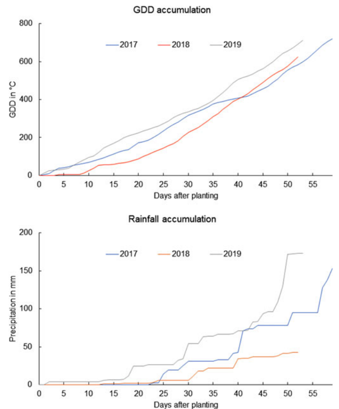
Fig. 3. Growing degree day (GDD) accumulation (top) and rainfall accumulation (bottom) from the day of CC planting to the day of CC termination for each year of the study.
