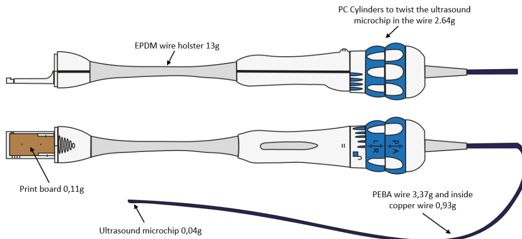
Figure 1. The ultrasound catheter investigated in this paper
