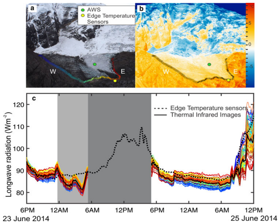
Fig. 5. Spatial variation of LW_{margin} . Each colored line on (a) is a location where surface temperature was extracted from the thermal infrared images for the 33 h of available imagery, at 5–10 min intervals. The same locations are thin black lines on the infrared images in (b). In (a) and (b), the green dot is the AWS, the yellow dot is the location of the edge temperature sensors and the W and E represent the west and east side of the ablation zone. In (c) each colored line is the LW_{margin\ discrete} at the corresponding color location in (a). The dashed black line is the longwave radiation calculated at the glacier margin with the edge temperature sensors and the thick black line is LW_{margin} , the average margin longwave flux from all the locations along the ablation zone from the infrared images. Only every third transect from (a) is shown for clarity. The light grey overlay delineates when weather conditions interfered with measurements and the dark grey overlay is when instrument malfunction prevented thermal infrared image acquisition.
