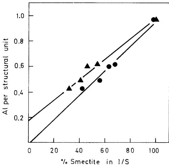
Figure 1. Uptake of Al by the clay vs. percentage of smectite layers as estimated by X-ray powder diffraction (●) and from K_{fix}/K_{fix,max} (▲).
