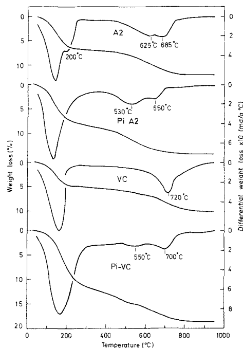
Figure 6. Thermogravimetric (TGA) and differential thermogravimetric (DTG) analyses of pillared montmorillonite, Pi-VC, pillared illite/smectite, Pi-A2, and the corresponding starting clays.
