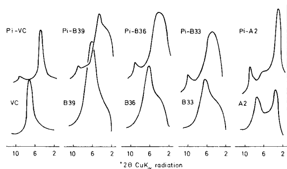
Figure 2. X-ray powder diffraction patterns of air-dried, oriented samples of pillared interstratified illite/smectite and the corresponding starting clays.
