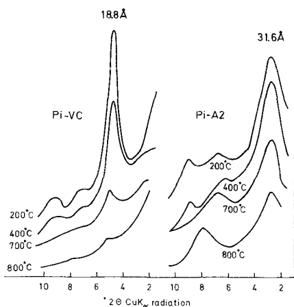
Figure 5. X-ray powder diffraction patterns of thermally treated samples of pillared montmorillonite, Pi-VC, and pillared illite/smectite, Pi-A2.
