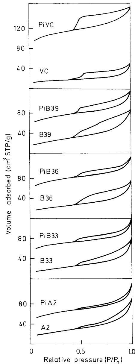
Figure 3. Nitrogen adsorption-desorption isotherms for pillared interstratified illite/smectite and the corresponding starting clays.
