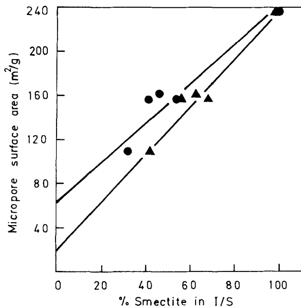
Figure 4. Micropore surface area of pillared illite/smectite as a function of smectite fraction in the starting clay, estimated by X-ray powder diffraction (●) and from K_{fx}/K_{fx,max} (▲).
