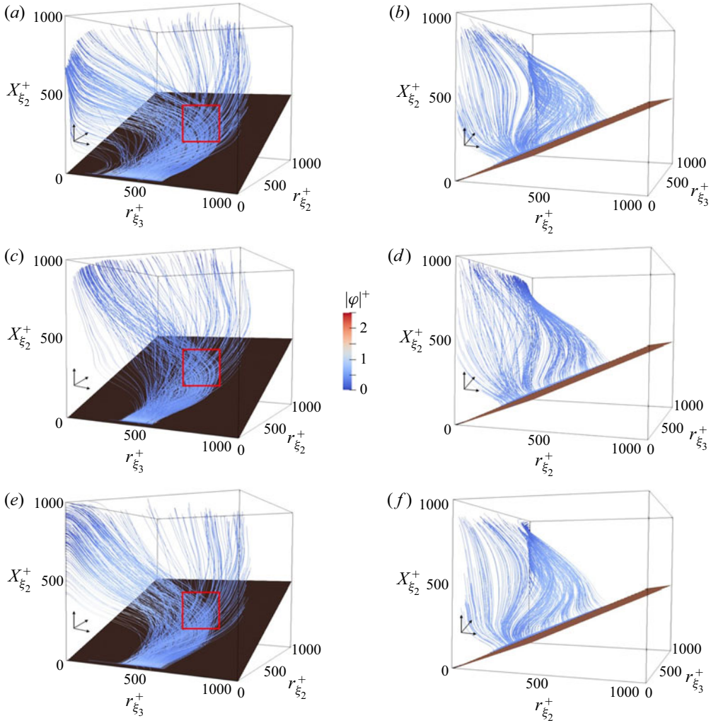
Figure 15. Scale-energy paths in the (r_{\xi_2}^+, r_{\xi_3}^+, X_{\xi_2}^+) space traced by means of the field lines of the flux vector field (\phi_{r_{\xi_2}^+}, \phi_{r_{\xi_3}^+}, \phi_{X_{\xi_2}^+}) for the rough-wall cases: (a,b) k^+ = 10 , \lambda^+ = 71 ; (c,d) k^+ = 60 , \lambda^+ = 424 and (e,f) the smooth-wall case at Re_\tau = 1080 . The r_{\xi_2}^+ - X_{\xi_2}^+ plane denotes the isosurface of the scale energy \langle \delta u' \delta u' \rangle = 0.05 . The colours scale according to the strength of flux vector field. The red square circle in (a–e) represents the energy transfer from small scale to large scale.
