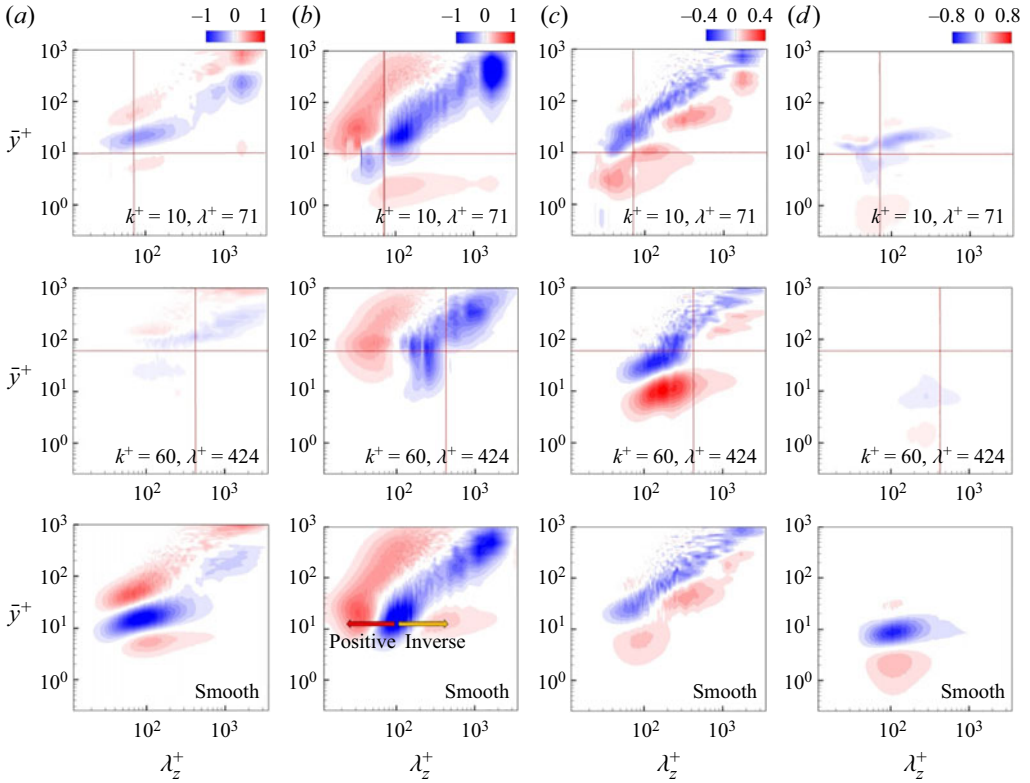
Figure 14. Contours of the one-dimensional pre-multiplied spanwise energy spectra of the spatial turbulent transport, scale-energy transport, viscous transport and pressure transport terms: (top) k^+ = 10, \lambda^+ = 71 ; (middle) k^+ = 60, \lambda^+ = 424 and (bottom) the smooth-wall case at Re_\tau = 1080 . Different terms, i.e. (a) T_{i,11}^{y+} , (b) T_{p,22}^{xz+} , (c) T_{v,11}^{+} and (d) T_{v,11}^{+} are presented. Red solid lines correspond to the wavelength and height of the roughness elements, respectively.
