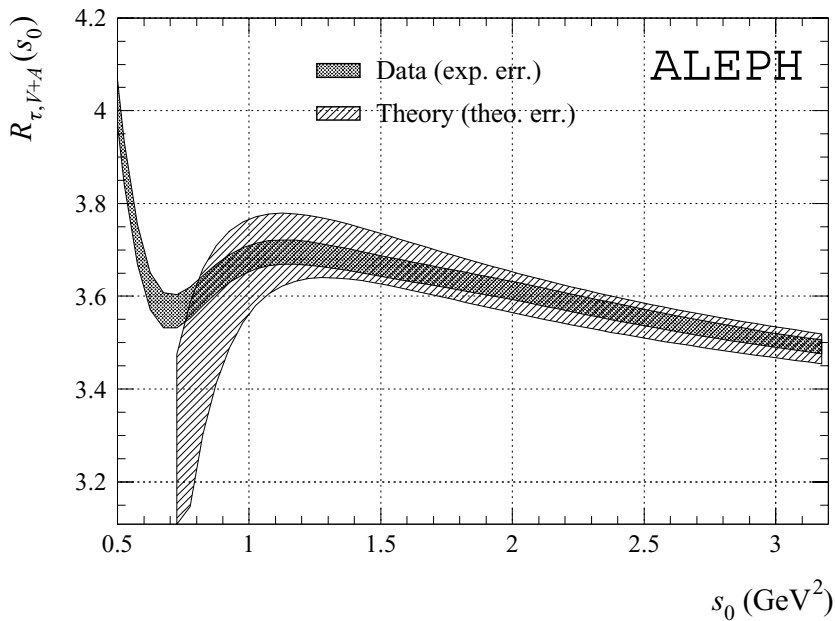
Fig. 25.9. R_{\tau,V+A} as a function of the \tau mass s_0 . The theoretical predictions are from FOPT.
