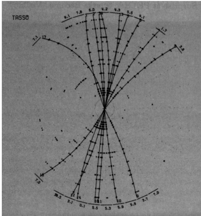
Fig. 24.3. Two-jet events seen in e + e - at PETRA (1979).
