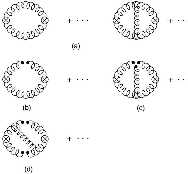
Fig. 37.1. Feynman diagrams corresponding to the OPE of the gluonium correlator: (a) perturbative; (b) two-gluon condensate; (c) three-gluon condensate; (d) four-gluon condensate.
