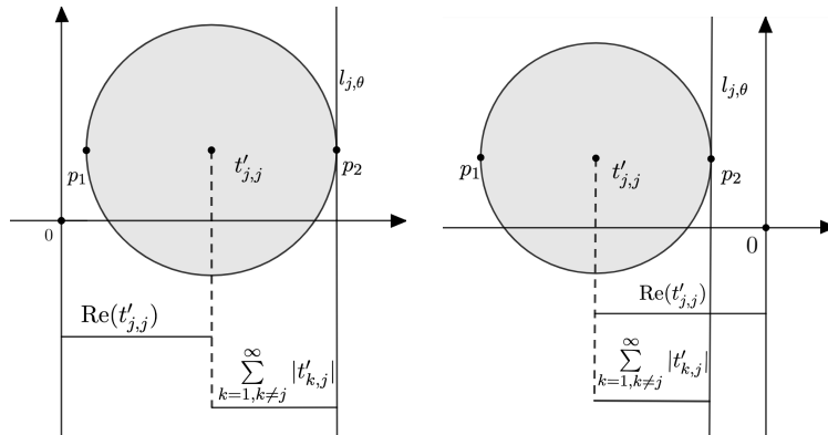
Figure 1: Illustration of the Gershgorin disk D(t'_{j,j}, \sum_{k=1, k \neq j}^{\infty} |t'_{k,j}|) together with the tangent line l_{j,\theta} . Its radius and the distance from 0 to its center is highlighted. The left picture shows an example when \text{Re}(t'_{j,j}) is positive and the right one corresponds to the negative case.
