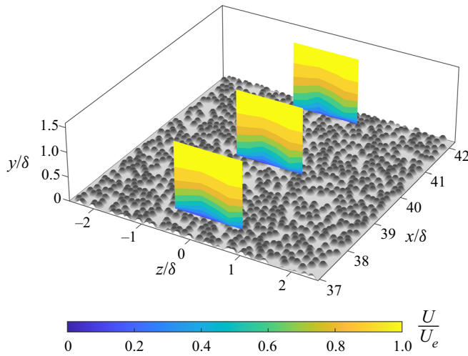
Figure 18. R78 mean streamwise velocity contour plot of three wall-normal spanwise planes in an isometric view. The centre plane is at x_0 = 1.50 m. The upstream and downstream planes are \pm 8 cm, approximately \pm 2\delta , from x_0 .
