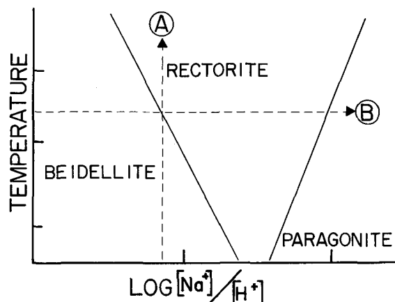
Fig. 12. Theoretical activity-temperature diagram for a Na-beidellite series. The pressure is one bar. Each stability field contains H_2O and quartz in addition to the phase shown.
