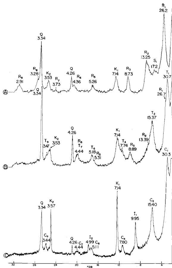
Fig. 9. Mg-montmorillonite series saturated with ethylene glycol. C is corrensite. I is illite. K is a kaolinitelike phase. Q is quartz. R is Mg-rectorite. S is unreacted smectite. T is tosudite. Pattern A is Mg-rectorite formed in run 26. Pattern B is Mg-rectorite and tosudite from run 27. Pattern C is a natural corrensite from a sandstone found in the Pecos Valley, New Mexico.
