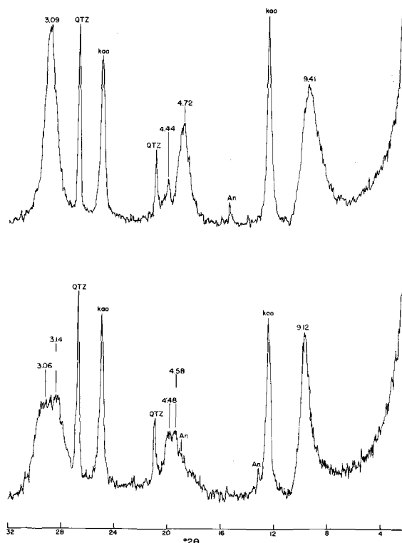
Fig. 11. Al-montmorillonite series. The products are from run 36. Air-dried sample is at top, ethylene glycol-treated at bottom. An is anorthite. Kao is kaolinite. Qtz is quartz. The other peaks are attributed to 25% expandable random pyrophyllite/smectite.
