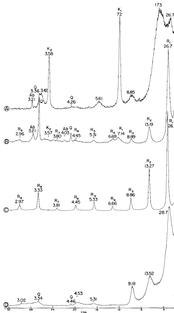
Fig. 7. Na-smectite series saturated with ethylene glycol. Ab is albite. K is kaolinite. Q is quartz. R is sodium rectorite. Peaks which have numbers only are attributed to Na-rectorite. Pattern A is a 70% expandable Na-rectorite formed in run 14. Pattern B is a 50% expandable Na-rectorite from run 15. Pattern C is a natural Na-rectorite from the Jeffrey Quarry, Arkansas. Pattern D is a 40% expandable Na-rectorite from run 17.
