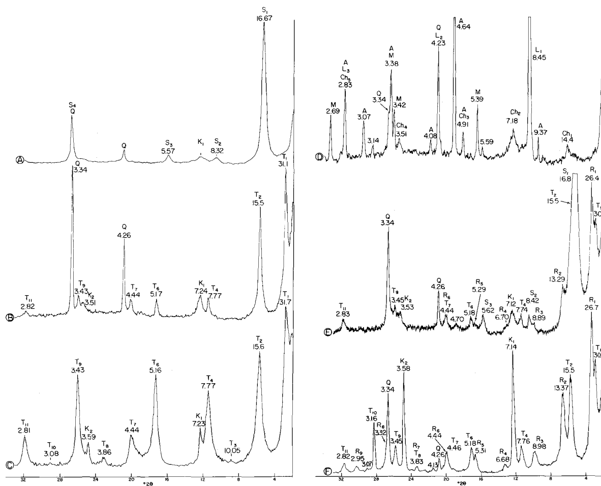
Fig. 8. Li-montmorillonite series saturated with ethylene glycol. A is an anthophyllitelike phase. Ch is a chlorite (cookeite?)like phase. K is kaolinite. L is an unidentified micalike phase. M is mullite. Q is quartz. R is a rectoritelike phase. S is smectite. T is lithium tosudite. Pattern A is a high charge smectite formed in run 19. Pattern B shows a Li-tosudite formed in run 20. Pattern C is a natural Li-tosudite from Huy studied by Brown et al. (1974). It is Ba-saturated. Pattern D shows products formed in run 23. Pattern E is Li-tosudite and rectorite formed in run 24. Pattern F is a natural Li-tosudite and rectorite (from the Roseki deposit) studied by Nishiyama et al. (1975).
