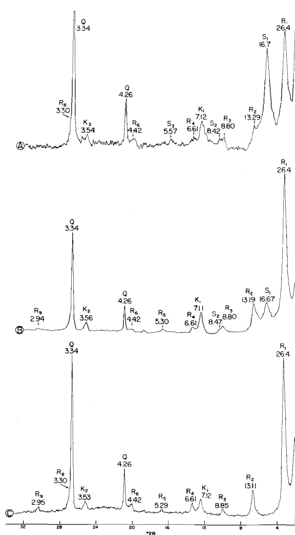
Fig. 10. Ca-montmorillonite series saturated with ethylene glycol. K is kaolinite. Q is quartz. R is Ca-rectorite. S is unreacted smectite. Pattern A shows Ca-rectorite formed in run 31. Pattern B is Ca-rectorite from run 32. Pattern C is Ca-rectorite from run 33.
