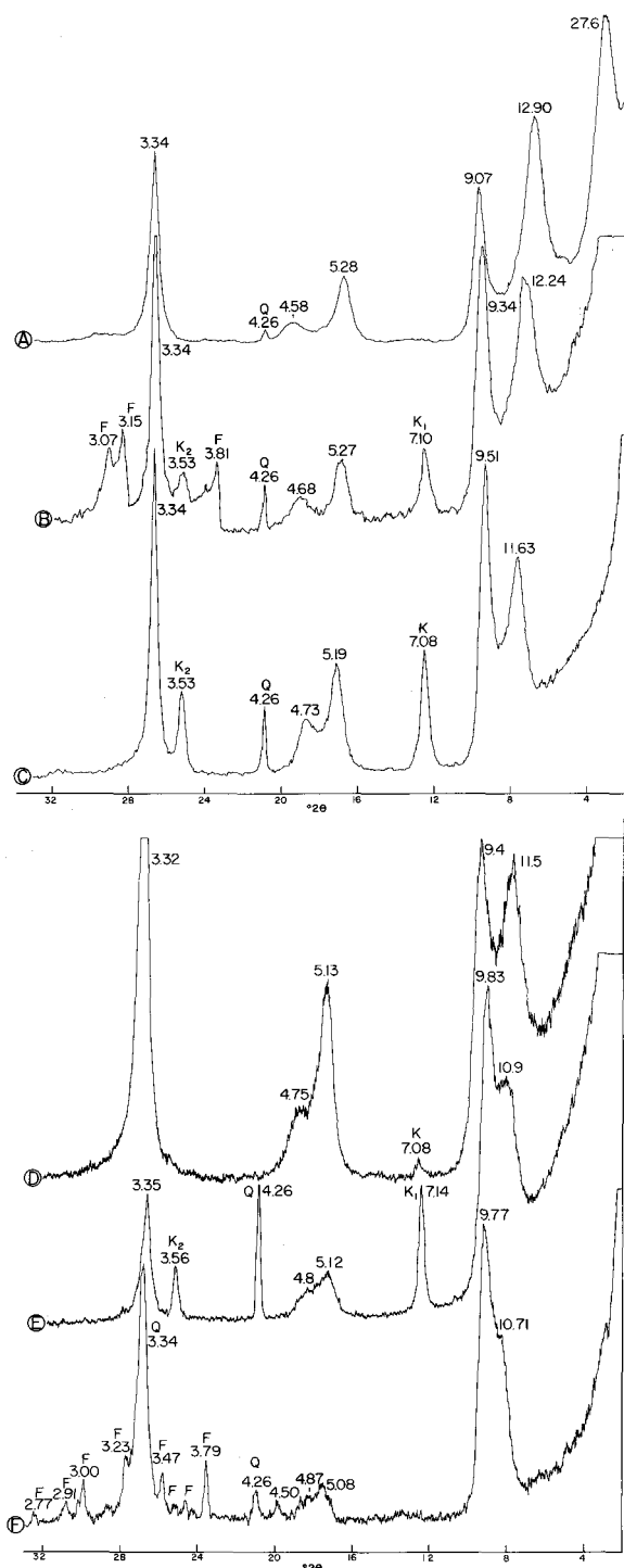
Fig. 6. K-montmorillonite subseries saturated with ethylene glycol. F is feldspar. The peaks which have numbers only are K-rectorites. Other symbols are given with Figure 1. Pattern A is a 40% expandable K-rectorite formed in run 6. Pattern B is 25% expandable K-rectorite from run 7. Pattern C is a 20% expandable K-rectorite from run 8. Pattern D is a natural K-rectorite (metabentonite) from the Ordovician Shoreham Formation of New York State. It is 15% expandable. Pattern E is an 11% expandable K-rectorite from run 10. Pattern F is a 7% expandable K-rectorite from run 11.
