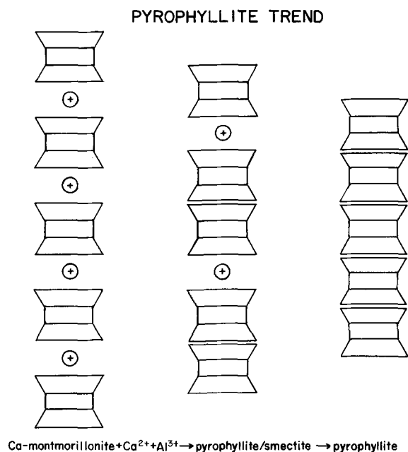
Fig. 3. Pyrophyllite trend. Symbols as in Figure 1.
