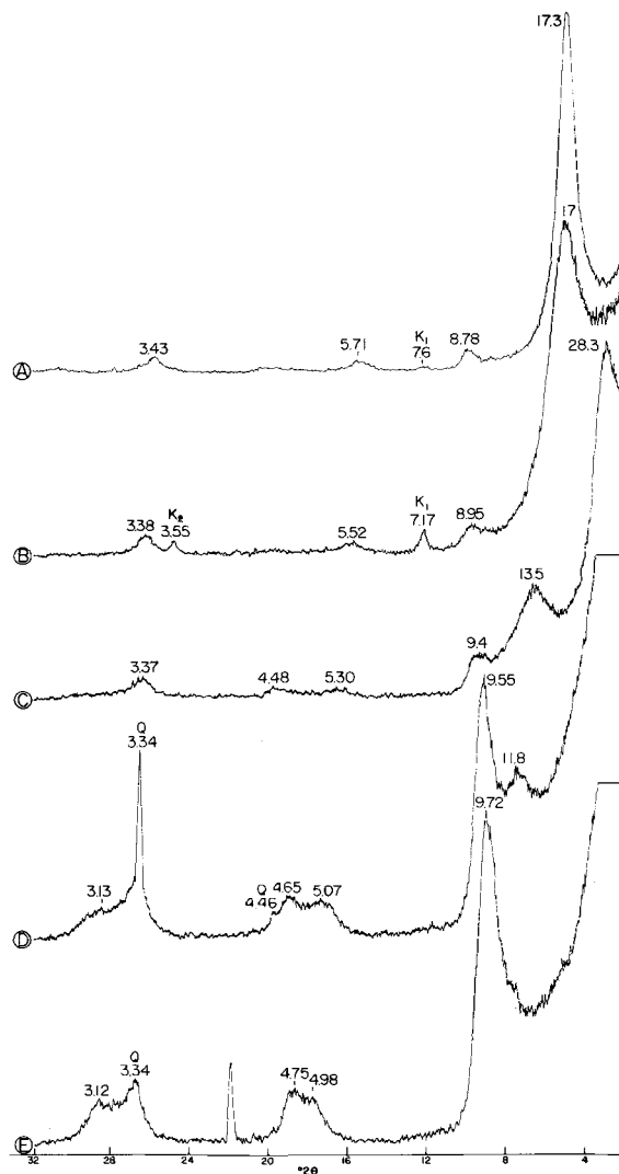
Fig. 5. K-beidellite subseries saturated with ethylene glycol. K is kaolinite. Q is quartz. The numbered peaks are attributed to mixed-layer illite/smectite. See Table 1 for run conditions. Pattern A is a 85% expandable random I/S formed in run 1. Pattern B is a 60% expandable random I/S formed in run 2. Pattern C is a 32% expandable K-rectorite formed in run 3. Pattern D is a 15% expandable K-rectorite from run 4. Pattern E is a 10% expandable IS from run 5. The peak between 20° and 24° is cristoballite.
