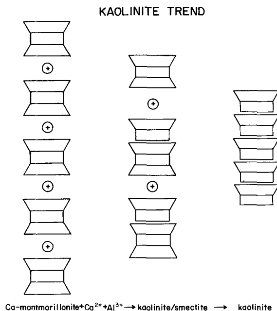
Fig. 4. Kaolinite trend. Symbols as in Figure 1.
