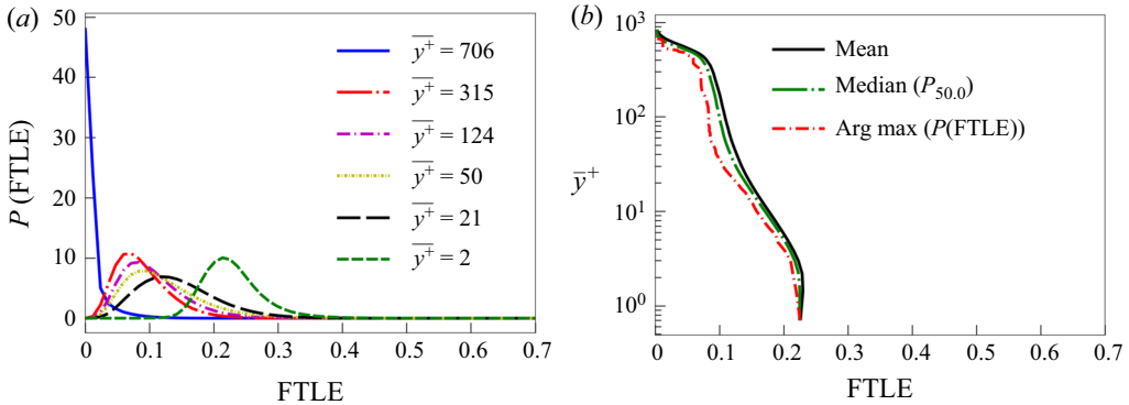
Figure 3. (a) Probability density functions (PDFs) of FTLE at different wall distances and (b) mean value, median of the FTLE and arg max of the PDF of the FTLE versus wall distance.
