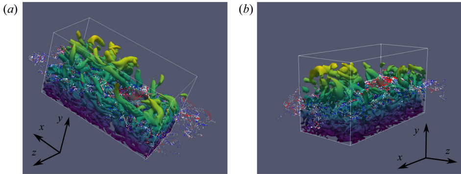
Figure 5. Comparison of particle positions from enlargement (a) in figure 4 with instantaneous vortices ( \lambda_2 = \text{const.} ).
