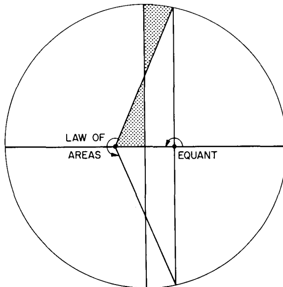
Fig. 4. The near-equivalence of the equant and the law of areas.
