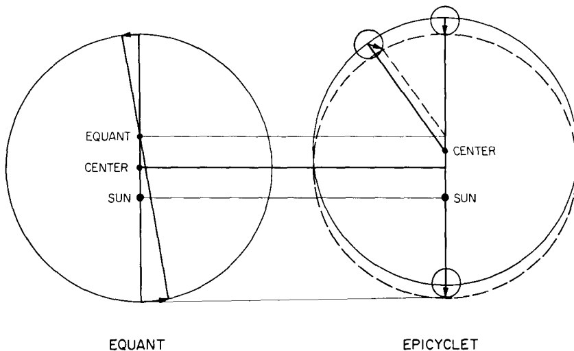
Fig. 5. Copernicus' replacement of the equant by a pair of uniform circular motions. The epicyclet has a radius of e/2 and always moves to form the isosceles trapezoid shown above.
