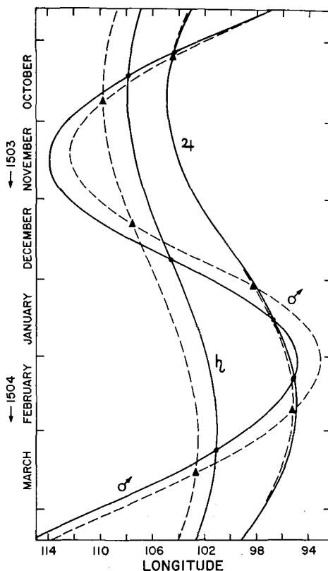
Fig. 2. Apparent motions of the superior planets just before the great conjunction of 1504. The solid lines and circles show the actual positions and conjunctions. The broken lines and triangles show the predicted positions and conjunctions.
