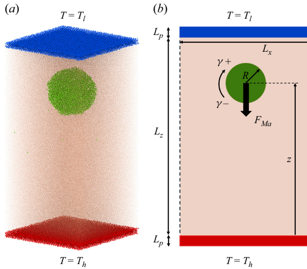
Figure 1. (a) A snapshot of a gas nanobubble in water between two solid plates in MD simulations. The top plate has a lower temperature T_l , and the bottom plate has a higher temperature T_h . (b) Sketch of a gas nanobubble in water between two solid plates. Here, \gamma is the local surface tension of the bubble surface, and the bubble portion with a lower (higher) temperature has a higher (lower) surface tension, denoted as \gamma+ ( \gamma- ). This creates a Marangoni flow around the bubble, resulting in a Marangoni force F_{Ma} on the bubble.
