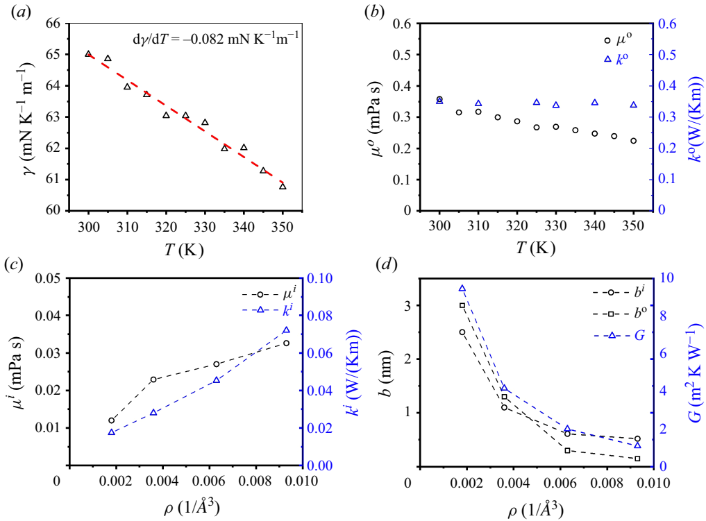
Figure 4. (a) Surface tension of the mW water model as a function of temperature. Symbols are MD results. The dashed lines show the linear fitting. (b) Viscosity (left-hand axis) and thermal conductivity (right-hand axis) for the mW water model. (c) Viscosity (left-hand axis) and thermal conductivity (right-hand axis) of gas as a function of gas density. (d) Liquid–gas slip (left-hand axis) and thermal resistance (right-hand axis) as a function of gas density.
