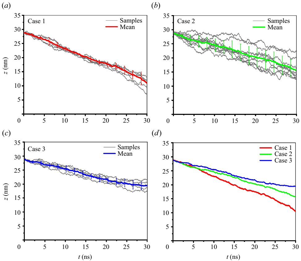
Figure 3. Trajectories of the moving bubbles in the molecular simulations for the three different cases. Grey lines represent different realizations in each case. The solid coloured lines are the mean trajectories of all the realizations, with the error bars representing the standard deviations: (a) case 1, bubble radius R = 5.0 nm and \Delta T = 50 K; (b) case 2, bubble radius R = 3.1 nm and \Delta T = 50 K; (c) case 3, bubble radius R = 5.0 nm and \Delta T = 25 K; (d) mean bubble trajectory for the mentioned three cases, for comparisons.
