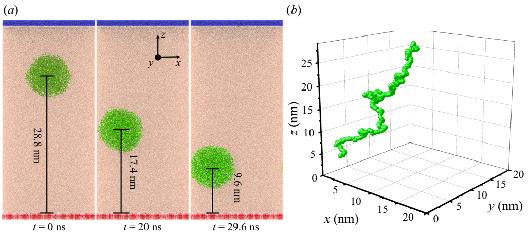
Figure 2. (a) Snapshots of the bubble movement in the MD simulations at three different times for case 1. (b) For the same simulation, the three-dimensional trace of the bubble motion is shown.
