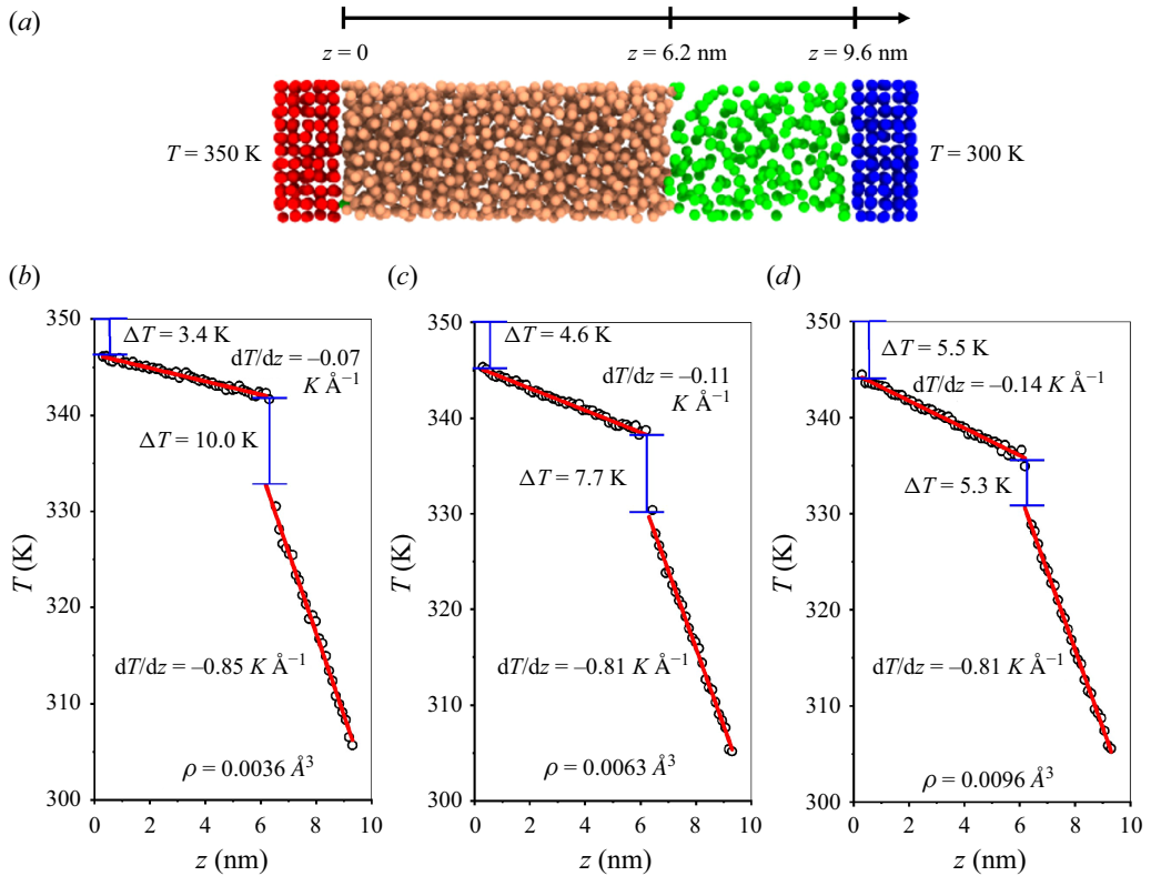
Figure 5. (a) Snapshot of the liquid–gas system in MD simulations to measure the liquid–gas thermal resistance. (b) The temperature profile for gas density 0.0036 \text{ \AA}^3 . (c) The temperature profile for gas density 0.0063 \text{ \AA}^3 . (d) The temperature profile for gas density 0.0096 \text{ \AA}^3 . The symbols are MD results, and the red lines are linear fittings.
