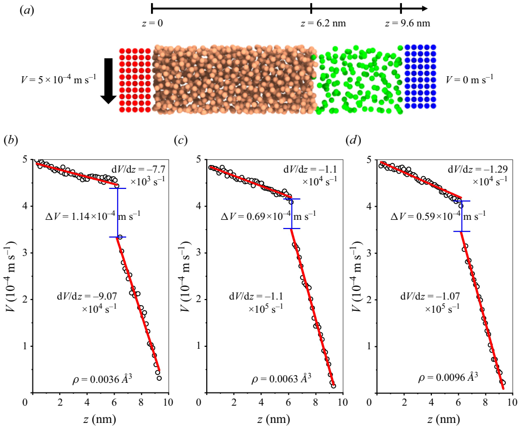
Figure 6. (a) Snapshot of the Couette flow to measure the gas–liquid slip. (b) The velocity profile for gas density 0.0036 \text{ \AA}^3 . (c) The velocity profile for gas density 0.0063 \text{ \AA}^3 . (d) The velocity profile for gas density 0.0096 \text{ \AA}^3 . The symbols are MD results, and the red lines are linear fittings.
