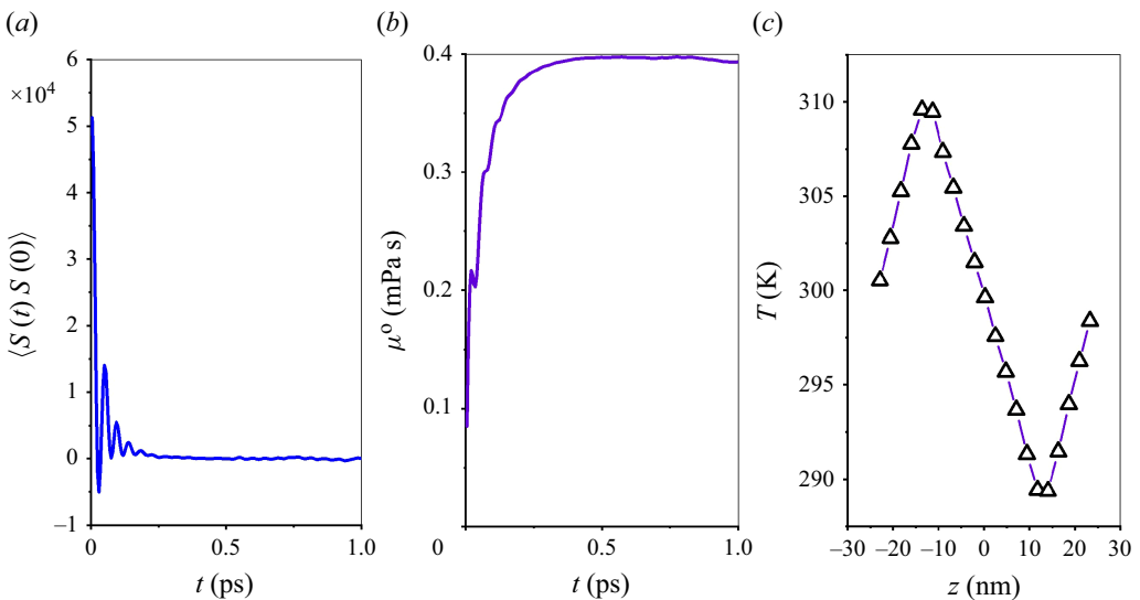
Figure 7. (a) Temporal correlations of the stress when measuring the mW water model with temperature 275.6 K. (b) Integrating the temporal correlation. (c) Temperature distribution in the heat flux method.
