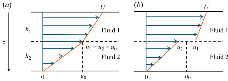
Figure 8. Two-phase Couette flow between two plates: (a) no-slip, (b) finite slip.
