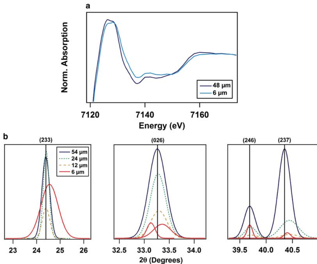
FIG. 4. (a) Representative Fe K -edge XANES spectra for almandine A both 6 \mu\text{m} adjacent to and 48 \mu\text{m} distant from an inclusion of zircon. (b) XRD traverse across almandine A surrounding the zircon inclusion. Assumed to have accumulated more radiation damage than almandine B, most XRD peaks across the track decrease in intensity and broaden into the irradiated region.
