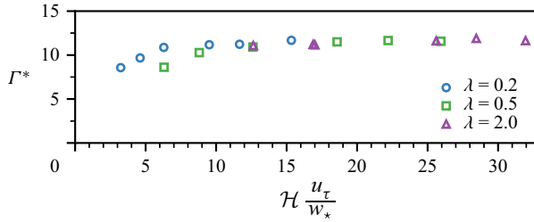
Figure 10. Datapoints for compensated circulation (see (3.2)) for the cases considered in this study (with the exception of case H, for which \Gamma^* = 0 ; see also table 1). Values of \Gamma^* are shown against \mathcal{H}(u_\tau/w_\star) = \Omega_B/\Omega_A (abscissa; see table 1 for case attributes) for the values of \lambda denoted in the figure.
