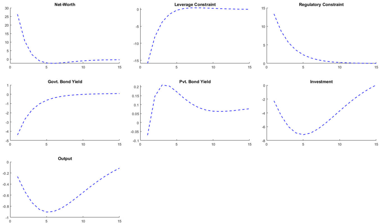
Figure 4. Impulse responses to a positive quantitative easing shock in the presence of credit regulations. Note: All variables are in percentage points and all rates are annualized.
