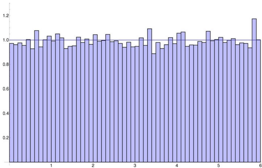
FIGURE 1. Pair correlation of \{(n - \sqrt{2})^2/2N\}_{n=1}^N \bmod 1 , with N = 5000 .
