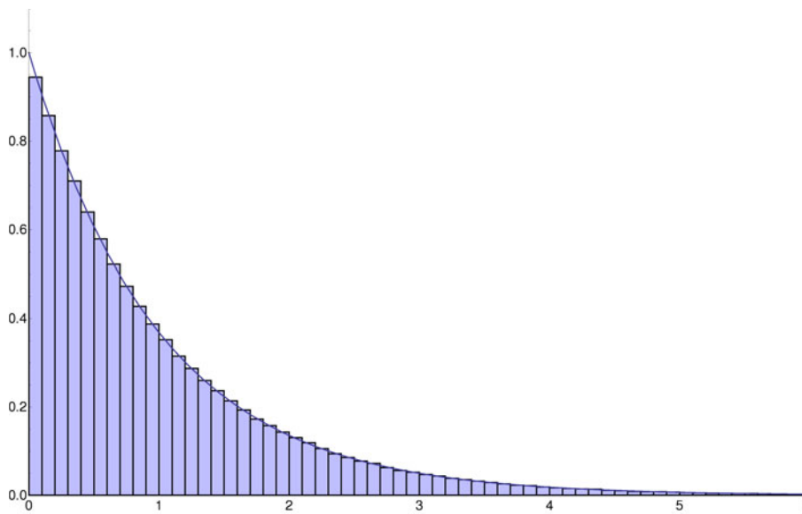
FIGURE 2. Gap distribution of \{(n - \sqrt{2})^2/2N\}_{n=1}^N \bmod 1 , with N = 10^6 .
