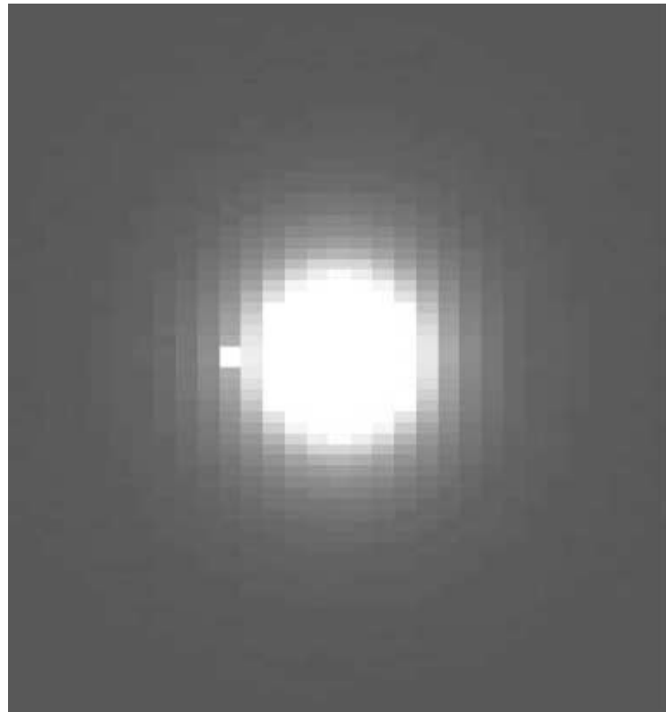
Figure 3 Simulated collapsed NIFS image showing a K = 18 mag companion star 0.5'' to the left of a K = 12 mag primary star in 0.4'' seeing with a Strehl ratio of 0.6. The exposure time with the K grating is 1800 s, which just saturates the K = 12 mag star.
