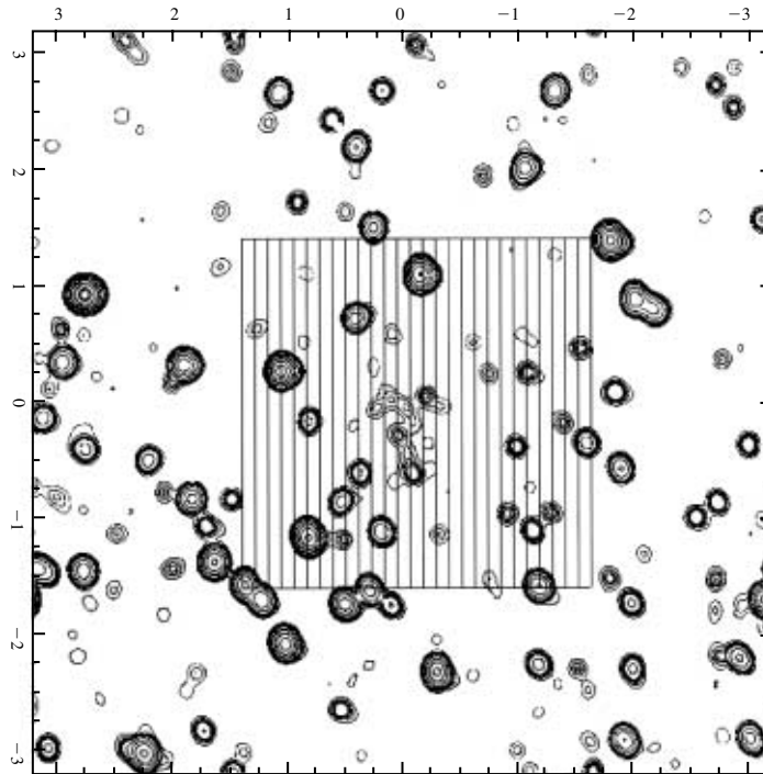
Figure 5 K -band image of the Galactic centre region (Eckart et al. 1995) centred on Sgr A*, the central black hole, with the NIFS field of view (square grid) superposed. The axis units are arcseconds on the sky.
