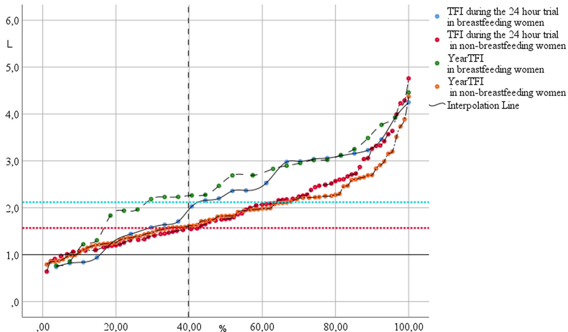
Fig. 2. Overlay scatterplot of individual total fluid intake in litre ( y -axis) split into breast-feeding and non-breast-feeding women. Percentiles on the x -axis. The two horizontal lines indicate the combined 40 percentile cut-off values of the 24 h trial (TFI) and estimates from the whole year (yearTFI) in non-pregnant, non-breast-feeding and breast-feeding women.
