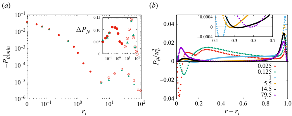
Figure 4. (a) Minimum of negative production ( -P_\theta|_{min} ) versus the inner radius; in the inset, the thickness \Delta P_N of the layer with P_\theta < 0 is plotted versus r_i . Red dots denote results obtained with the r v_\theta -formulation, red circles with the v_\theta -formulation, and green triangles with the GPU-version of the v_\theta -formulation. (b) Profiles of TKE production scaled by bulk velocity versus distance from the inner wall; the inset shows a close-up view of the production profiles for flow cases with r_i > 1 . The values of r_i are reported in the legend. Both plots refer to azimuthal flows.
