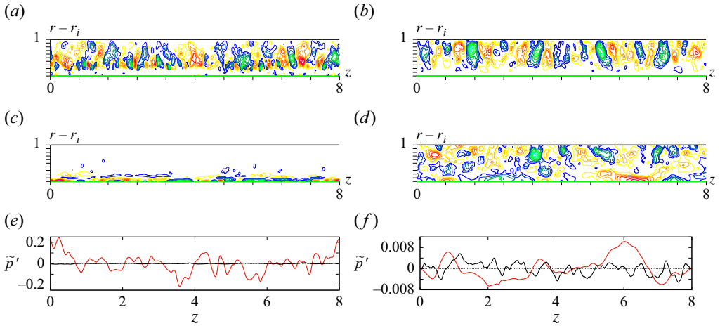
Figure 9. Contours in transverse ( r - z ) planes of azimuthal flow cases with (a,c) r_i = 0.025 and (b,d) r_i = 1 . Fluctuating radial velocity \tilde{v}'_r scaled with the maxima (a) \tilde{v}'_{r,max} = -0.25 and (b) \tilde{v}'_{r,max} = -0.128 . Pressure \tilde{p}' scaled with the maxima (c) \tilde{p}'_{max} = 0.26 and (d) \tilde{p}'_{max} = -0.0137 . The outer wall is at the top, and the inner wall is at the bottom of each plot. Blue, green, cyan represent negative values, and yellow, red, magenta represent positive values, with increments \Delta = 0.1 . Profiles of \tilde{p}' on the inner wall (red) and outer wall (black) of (e) r_i = 0.025 and (f) r_i = 1 .
