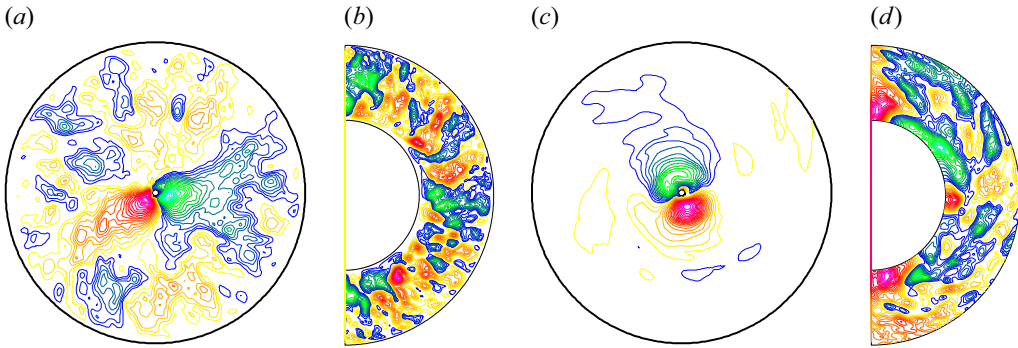
Figure 11. Contours in longitudinal ( \theta - r ) planes of azimuthal flow cases with (a,c) r_i = 0.025 and (b,d) r_i = 1 , and fluctuating (a,b) radial velocity \tilde{v}_r and (c,d) pressure p' , both averaged along the z -direction, scaled by their maximum values: (a) \widehat{v}_{r_{max}} = 0.053 , (b) \widehat{v}_{r_{max}} = 0.026 , (c) \widehat{p}'_{max} = 0.092 , (d) \widehat{p}'_{max} = 0.006 . Blue, green, cyan represents negative values, and yellow, red, magenta represent positive values, with increments \Delta = 0.05 . Mean flow is clockwise.
