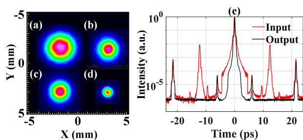
Figure 5. (a)–(d) Near-field beam profiles of the input, after passing one plate in stage 1 and four plates in stage 1, and the output. (e) SAC intensities of the input and output pulses.
