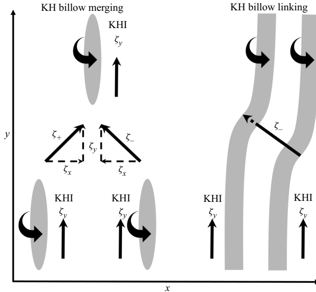
Figure 5. Idealized examples of misaligned KH billows (grey with \zeta_y > 0 ) enabling merging and linking (left and right) and emerging vortex tubes (slanted arrows) labelled \zeta_- and \zeta_+ both have \zeta_y > 0 (labelled with respect to their component vorticity along x ) driving knot dynamics thereafter. Vortex tubes arise on the intermediate vortex sheets due to differential stretching where the KH billows are misaligned along y . Note the 90^\circ rotation relative to figure 3. The left and right cartoons correspond to the knots and tubes, respectively.
