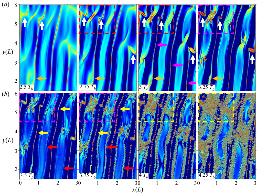
Figure 8. As in figure 7 at top for sub-sections of the \zeta(x, y) fields from 2.5\text{--}4.25T_b at 0.25T_b intervals. See text for discussion of the highlighted features. Turbulence onset is considered to accompany the rapid emergence of resolved, but much smaller, vortices. Also see the discussion of figures 14 and 15 below.
