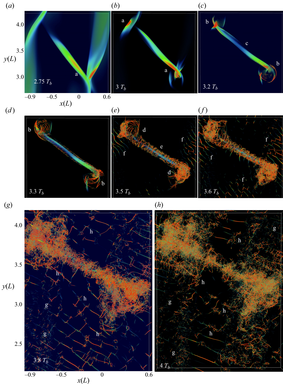
Figure 12. As in figure 11 for \lambda_2 from 2.75-4T_b viewed from above spanning the interval of strong initial KH billow and tube interactions and initial knot dynamics. Earlier times are shown in the larger y portion of Region 2. Labels denote features described in § 4.3.1.
