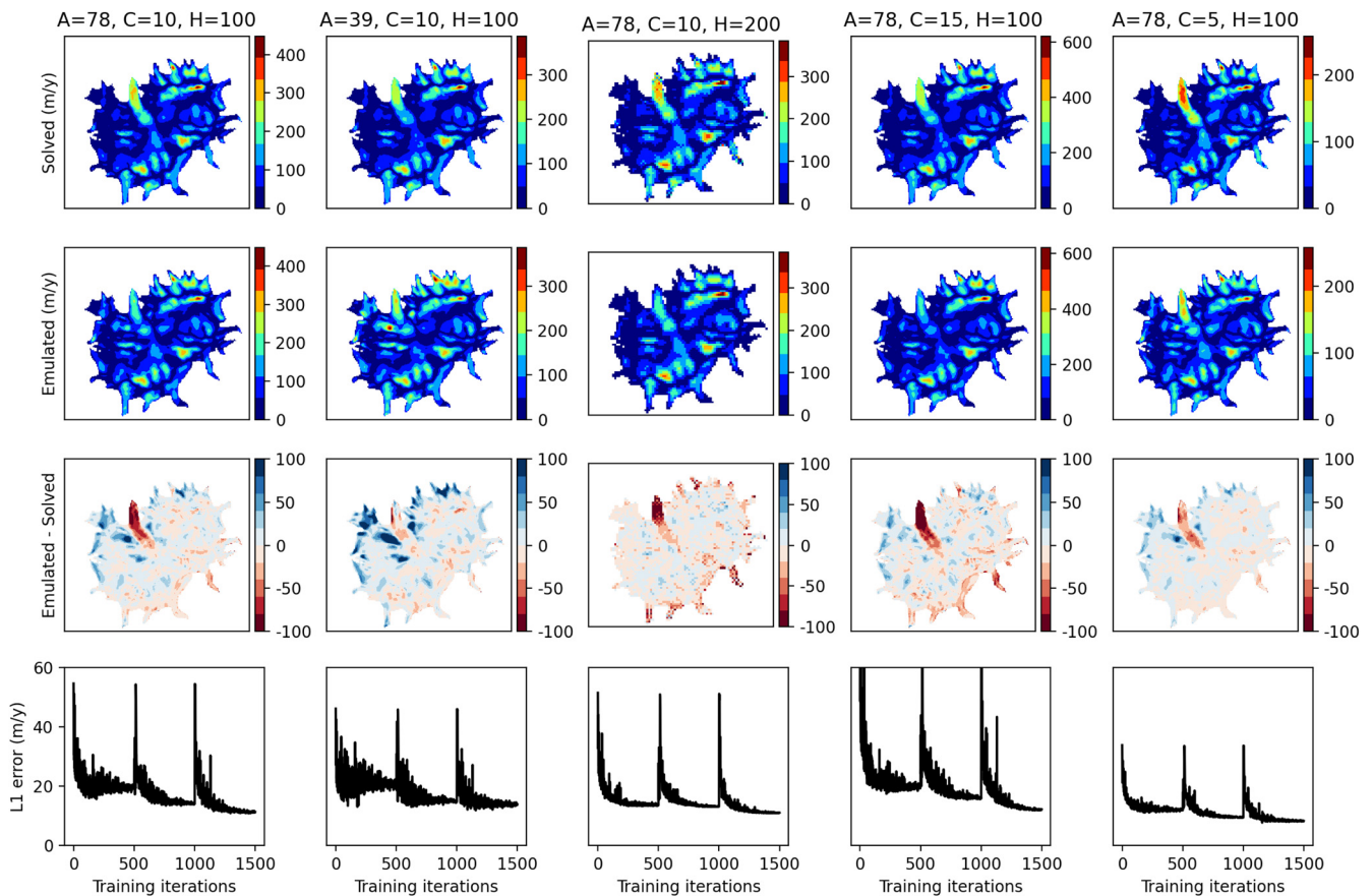
Figure A4. Results of the emulator on the ‘test’ glacier with varying values of A , c and H . Each column corresponds to one parameter set (A, c, H) (the first column shows the default original parameters). The first row displays the ‘solved’ surface ice-flow solution. The second row displays the ‘emulated’ solution after training over the glacier catalogue, while the third shows the difference between this solution and the ‘solved’ one. The last row shows the L1 error through the training. The jumps each 5000 iterations are due to the re-initialization of the learning rate.
