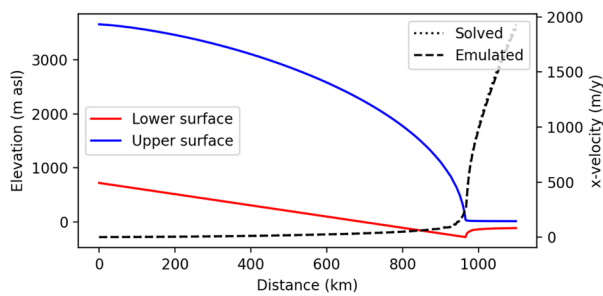
Figure 11. MISMIP-inspired ice geometry of the ice-shelf experiment along the x -axis, and resulting ice-flow velocities modelled from the solver and the emulator with custom training on the specific geometry.
