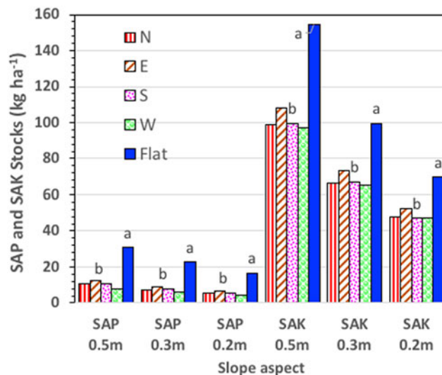
Figure 7. Soil available phosphorous (SAP) stocks and soil available potassium (SAK) stocks for 0.2, 0.3 and 0.5 m depth layers depending on slope aspect.
