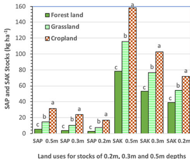
Figure 3. Soil available phosphorous (SAP) stocks and soil available potassium (SAK) stocks for 0.2, 0.3 and 0.5 m depth layers in the three land uses; different letters in a grouping mean significantly different using Duncan’s multiple range test.
