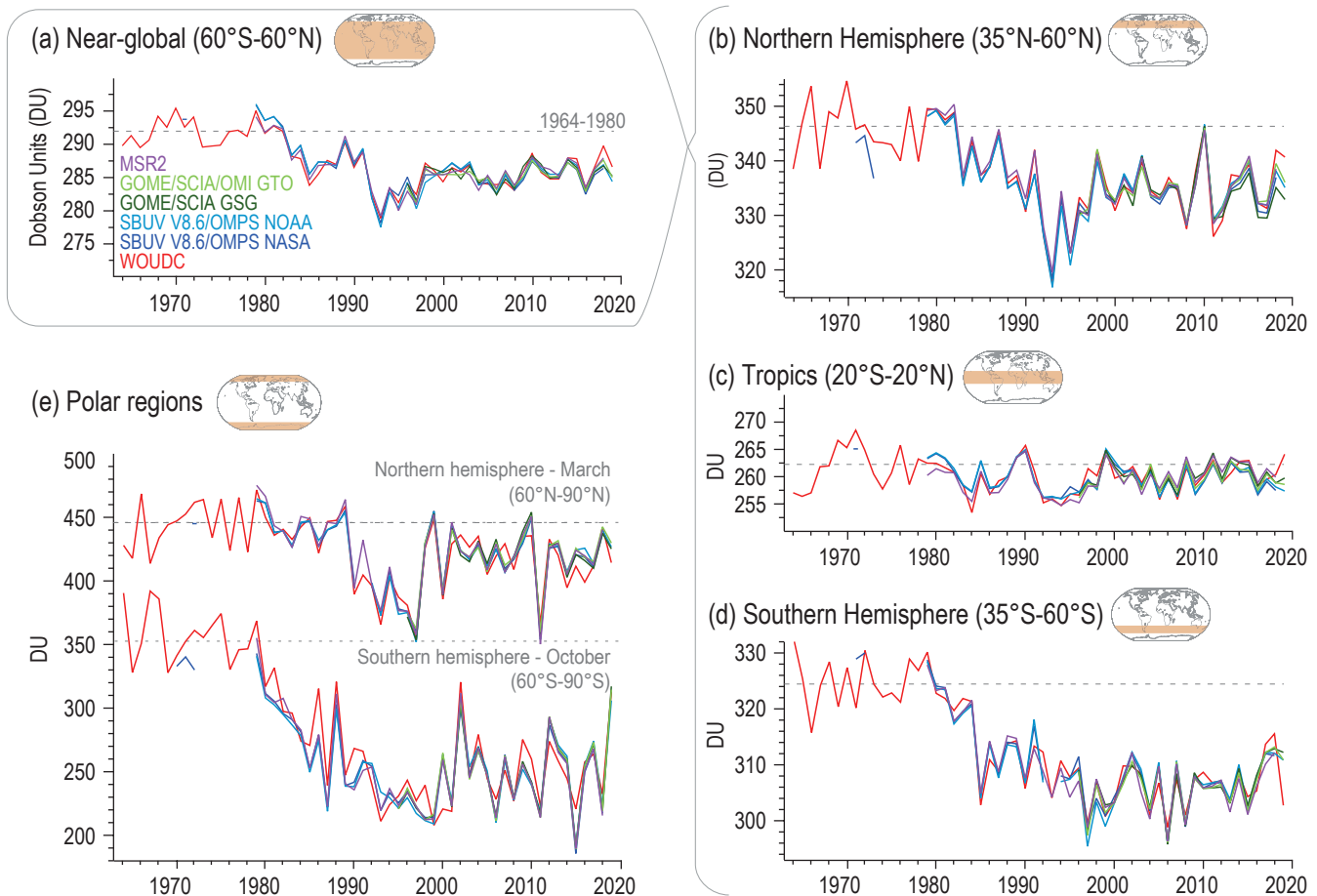
Mean total ozone in six regions
