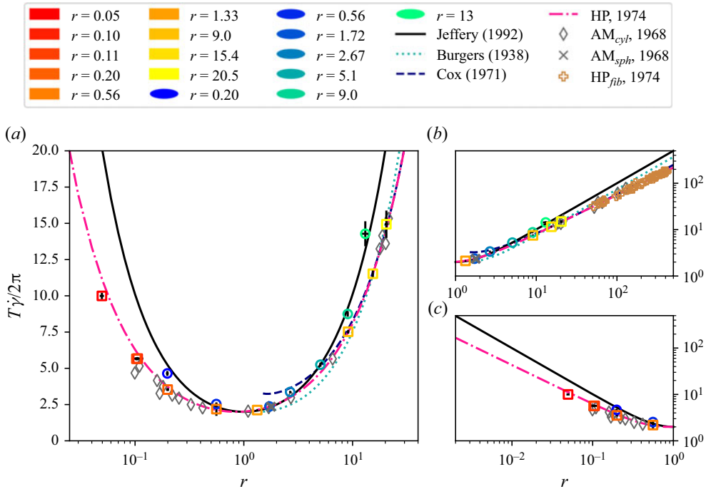
Figure 7. Period of rotation, T , of the axisymmetric particles against the particle aspect ratio r . The period is made dimensionless using the shear rate \dot{\gamma} and normalised by a factor 2\pi . (a) Both prolate and oblate, (b) prolate and (c) oblate particles. The experimental values are displayed as coloured rectangles (cylindrical particles) and circles (spheroidal particles). Each point is the average over all the available experiments for all particle Reynolds numbers ( Re_p \lesssim 1 ). The theories of Jeffery (1922) and Burgers (1938), the semi-empirical correlation of Cox (1971) and the empirical expression of Harris & Pittman (1975) are displayed as a solid black line, a dotted cyan line, a dashed blue line and a dash-dotted pink line, respectively. The experiments of Anczurowski & Mason (1968) are displayed as empty grey diamonds (cylinders) and one solid \times (spheroid), while the data of Harris & Pittman (1975) correspond to empty brown plus symbols. See supplementary materials for the directory of the figure including the data and the Jupyter notebook, https://www.cambridge.org/S0022112023010078/JFM-Notebooks/files/fig7/fig7.ipynb .
