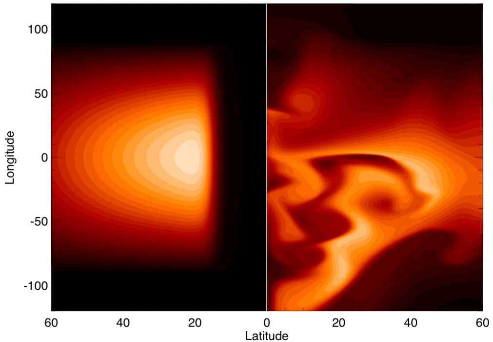
Figure 1. Initial temperature distribution (left) and after 15 orbital period (right).
