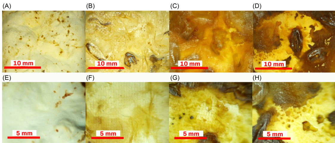
Figure 5. Mycelium samples include; A) and E) Set 10 untreated control, B) and F) Set 3 Glycerol 30% w/w (24 hours), C) and G) Glycerol 30% w/w (24 hours) + Tanner 6 hours, D) and H) Glycerol 30% w/w (24 hours) + Tanner 24 hours. Magnification levels shown in images A-D are 0.5X and 2.5X in images E-H.
