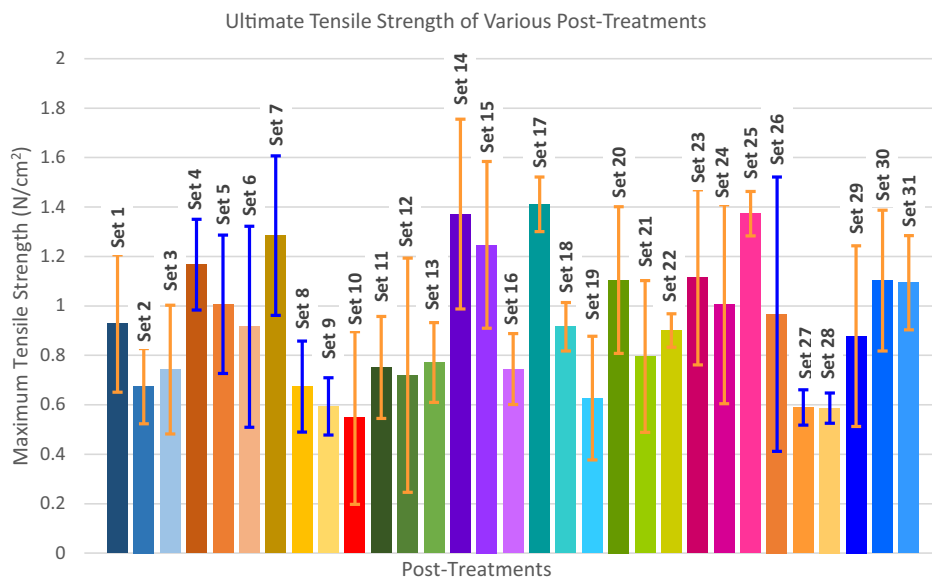
Figure 7. Ultimate tensile strength of post-treatments: Set 1 Glycerol 10% w/w (24 hours) (mean StDev = 0.278), Set 2 Glycerol 20% w/w (24 hours) (mean StDev = 0.152), Set 3 Glycerol 30% w/w (24 hours) (mean StDev = 261), Set 4 Glycerol 10% w/w (24 hours) + Tanner 6 hours (mean StDev = 0.183), Set 5 Glycerol 20% w/w (24 hours) + Tanner 6 hours, Set 6 Glycerol 30% w/w (24 hours) + Tanner 6 hours (mean StDev = 0.406), Set 7 Glycerol 10% w/w (24 hours) + Tanner 24 hours (mean StDev = 0.322), Set 8 Glycerol 20% w/w (24 hours) + Tanner 24 hours (mean StDev = 0.184), Set 9 Glycerol 30% w/w (24 hours) + Tanner 24 hours (mean StDev = 0.116), Set 10 None (Control), Set 11 Glycerol 10% w/w (48 hours) (mean StDev = 0.349), Set 12 Glycerol 20% w/w (48 hours) (mean StDev = 0.474), Set 13 Glycerol 30% w/w (48 hours) (mean StDev = 0.161), Set 14 Glycerol 10% w/w (48 hours) + Tanner (6 hours) (mean StDev = 0.384), Set 15 Glycerol 20% w/w (48 hours) + Tanner (6 hours) (mean StDev = 0.337), Set 16 Glycerol 30% w/w (48 hours) + Tanner (6 hours) (mean StDev = 0.143), Set 17 Glycerol 10% w/w (48 hours) + Tanner (24 hours) (mean StDev = 0.110), Set 18 Glycerol 20% w/w (48 hours) + Tanner (24 hours) (mean StDev = 0.098), Set 19 Glycerol 30% w/w (48 hours) + Tanner (24 hours) (mean StDev = 0.250), Set 20 Citric Acid 5 g/L w/w (24 hours) + 30% Glycerol + 10g Epsom/L (1 hr) (mean StDev = 0.297), Set 21 Citric Acid 10 g/L w/w (24 hours) + 30% Glycerol + 10 g Epsom/L (1 hr) (mean StDev = 0.307), Set 22 Citric Acid 15 g/L w/w (24 hours) + 30% Glycerol + 10 g Epsom/L (1 hr) (mean StDev = 0.068), Set 23 Citric Acid 5 g/L w/w (24 hours) + 10% Glycerol (mean StDev = 0.354), Set 24 Citric Acid 10 g/L w/w (24 hours) + 10% Glycerol (mean StDev = 0.403), Set 25 Citric Acid 15g/L w/w (24 hours) + 10% Glycerol (mean StDev = 0.090), Set 26 Citric Acid 5 g/L w/w (24 hours) + 20% Glycerol (mean StDev = 0.555), Set 27 Citric Acid 10 g/L w/w (24 hours) + 20% Glycerol (mean StDev = 0.071), Set 28 Citric Acid 15 g/L w/w (24 hours) + 20% Glycerol (mean StDev = 0.061), Set 29 Citric Acid 5 g/L w/w (24 hours) + 30% Glycerol (mean StDev = 0.366), Set 30 Citric Acid 10 g/L w/w (24 hours) + 30% Glycerol (mean StDev = 0.284), Set 31 Citric Acid 15 g/L w/w (24 hours) + 30% Glycerol (mean StDev = 0.191).
