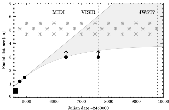
Figure 2. Radial location of the expanding sphere of crystal-rich dust as predicted by our modeling. The black square is the outburst in 2008, the two data points around JD~4700 and 4900 are the Spitzer Space Telescope observations in 2008 October and 2009 April, while the lower limits are our MIDI and VISIR measurements. Asterisks mark the location of the water snowline. The shaded area is the probable location of the crystalline forsterite grains.
