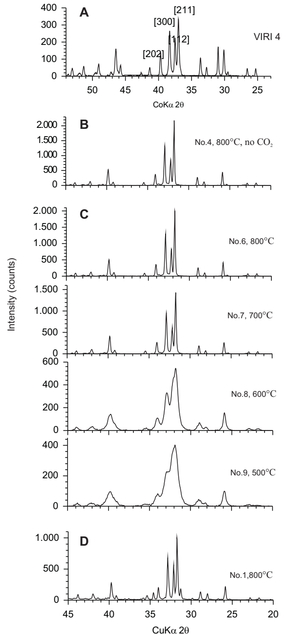
Figure 4 Selection of XRD powder pattern of: A) archaeological cremated bone from the VIRI intercomparison (VIRI sample 4, Naysmith et al. 2007); B) cremated bone material without old CO 2 (wet conditions); C) cremated and burnt bone with old CO 2 from 500 °C–800 °C (wet conditions); and D) cremated bone material with old CO 2 at 800 °C (dry conditions). Typical XRD peaks for hydroxylapatite crystal planes are indicated in the upper panel.
