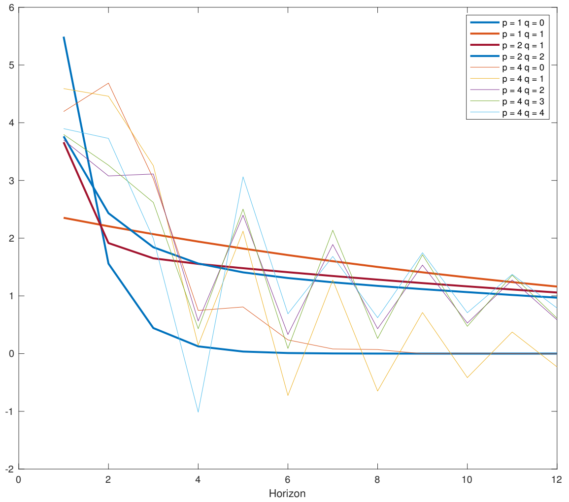
Figure 8: Impulse Response Functions for VRP on selected ARMA specifications.
