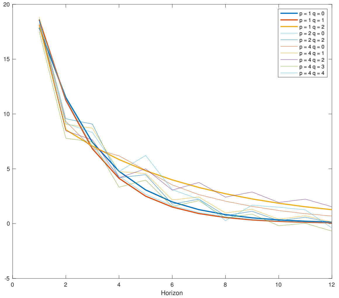
Figure 9: Impulse Response Functions for RV on selected ARMA specifications.
