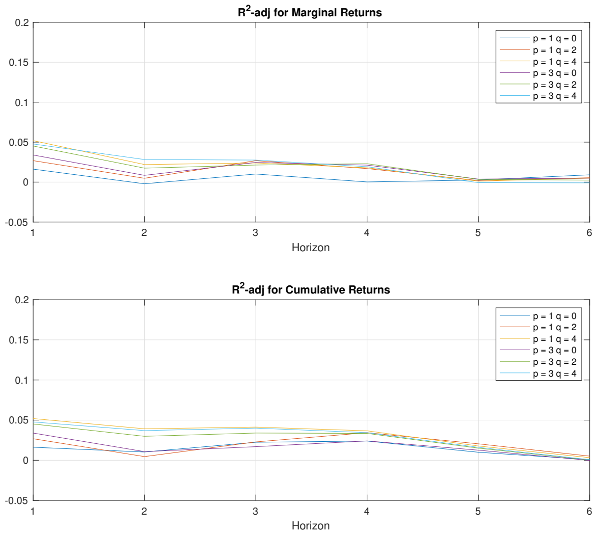
Figure 6: RV R^2 's for predictability regressions up to six months using ARMA components.
