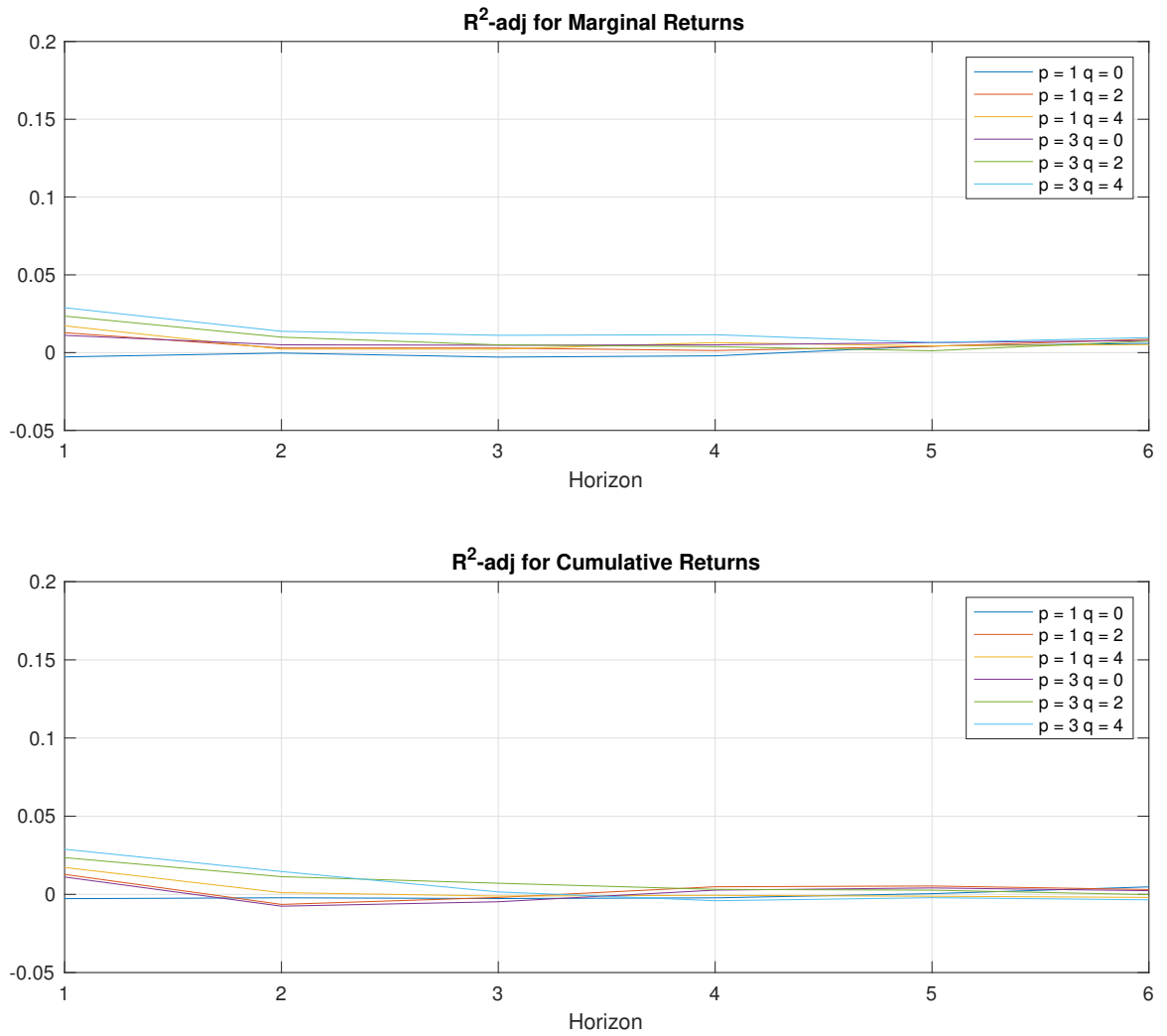
Figure 5: IV R^2 's for predictability regressions up to six months using ARMA components.
