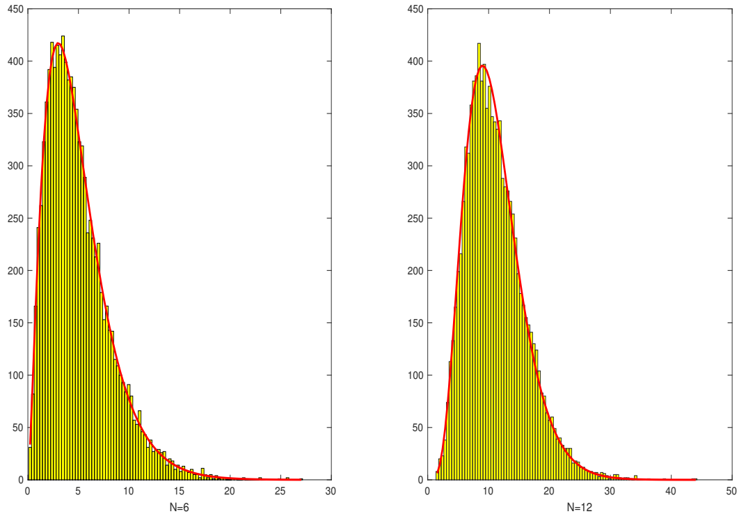
Figure 2: Distribution of Q_N under parameter values as in Table 1, T = 348 for N = 6 and 12 and \chi^2(5) and \chi^2(12) densities respectively.
