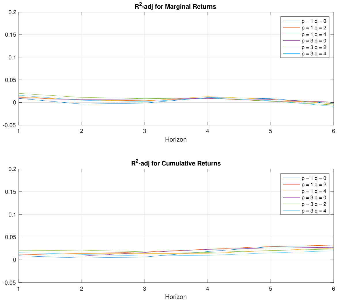
Figure 7: TI R^2 's for predictability regressions up to six months using ARMA components.
