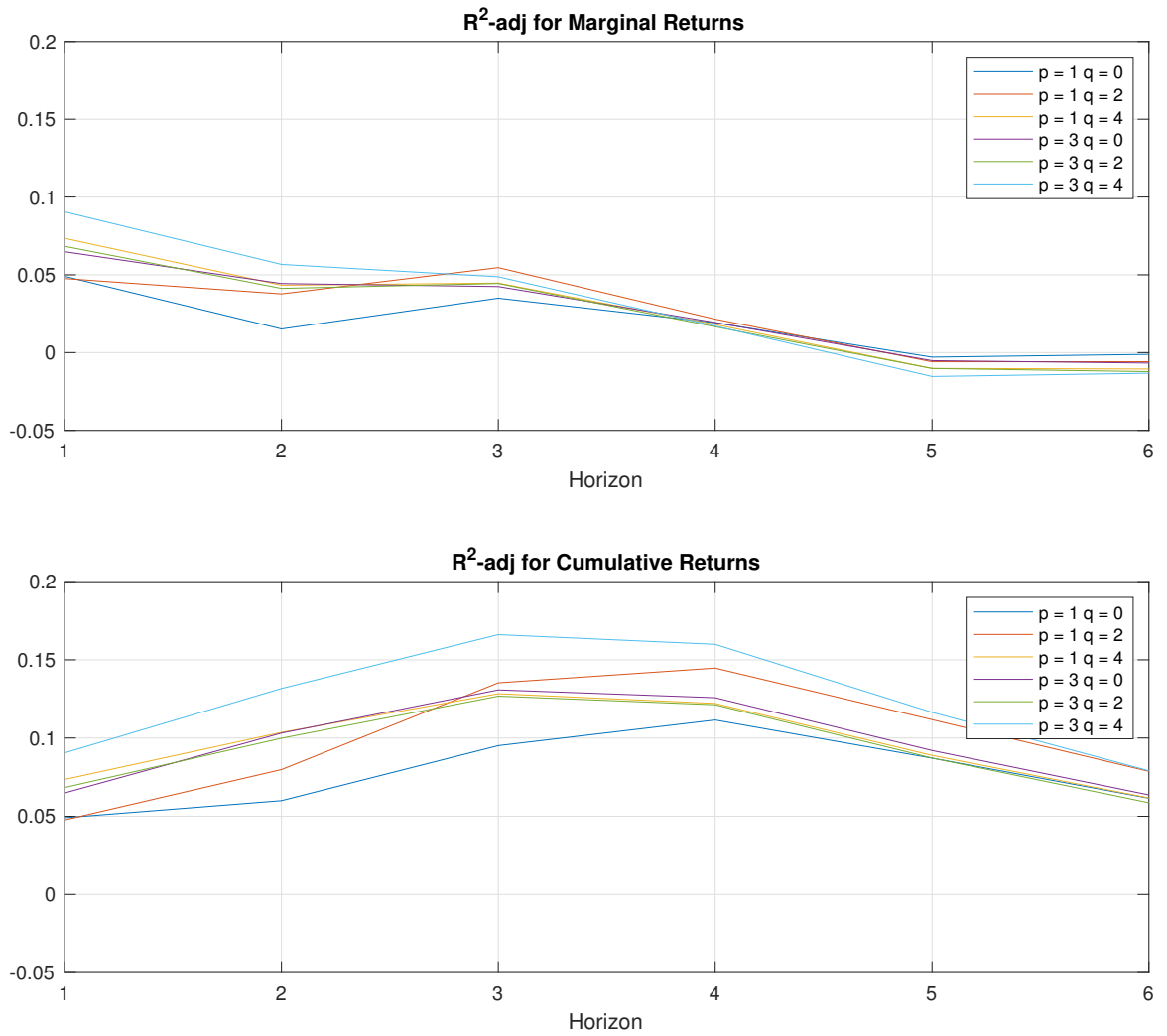
Figure 4: VRP R^2 's for predictability regressions up to six months using ARMA components.
