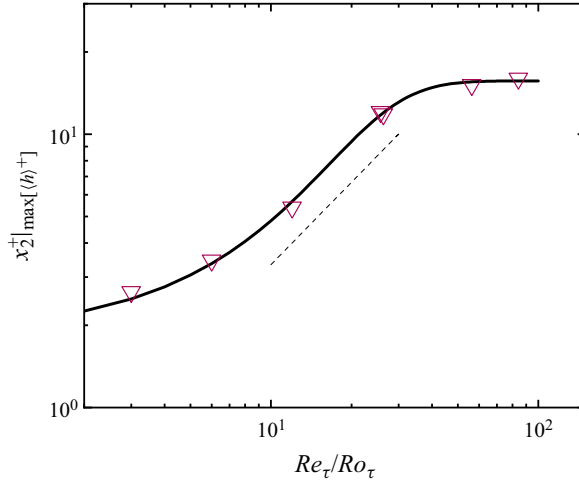
Figure 3. Relation between the peak x_2^+ |_{\max\{h\}^+} and the parameter Re_\tau / Ro_\tau . The black solid line is the fitted sigmoid function (2.4) and the black dashed line serves as a reference for the linear law.
