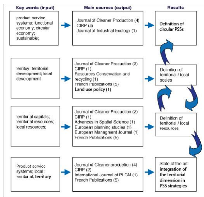
Figure 1. Research model
