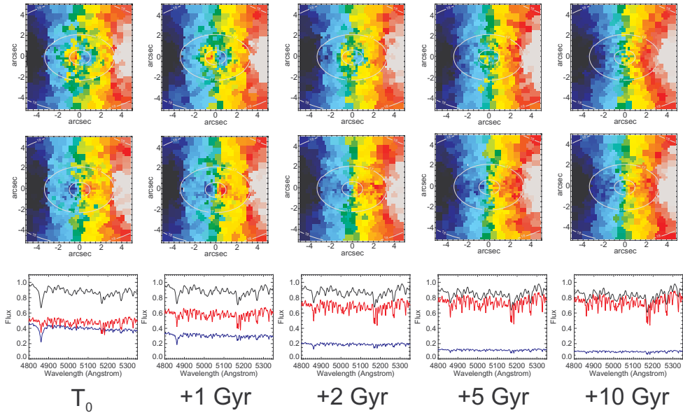
Figure 2. Model velocity fields for a counter-rotating (top row) and co-rotating (middle row) young subcomponent. The spectrum of the young component (blue - lower) and older main component (red - middle) are shown on the bottom row, indicating their luminosity-weighted contribution to the observed spectrum (black).
