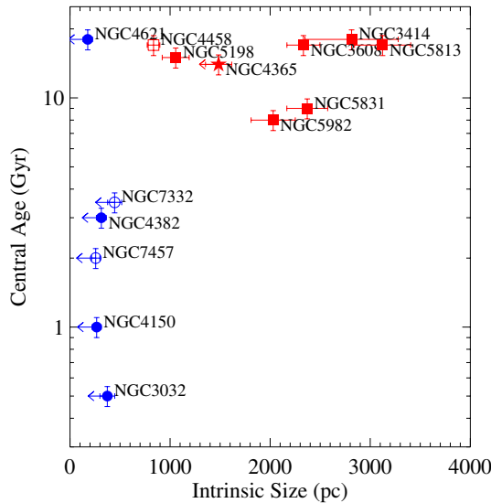
Figure 1. Intrinsic size of KDCs versus their central luminosity-weighted age. Closed symbols show objects observed by both SAURON and OASIS. Open symbols show objects only observed with SAURON. Red squares indicate slow-rotators and blue circles indicate fast rotators, as defined in Emsellem et al. ( submitted ). Arrows indicate where the measured diameter of the KDC is less than four times the seeing FWHM, implying that the KDC is not well-resolved and may be smaller than measured here.
