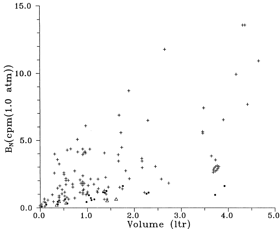
Fig. 1. Comparison of background in gas proportional counters. + - ordinary counters in surface laboratories; • - counters in underground laboratories; \Delta - counters in Trondheim dating laboratory.
