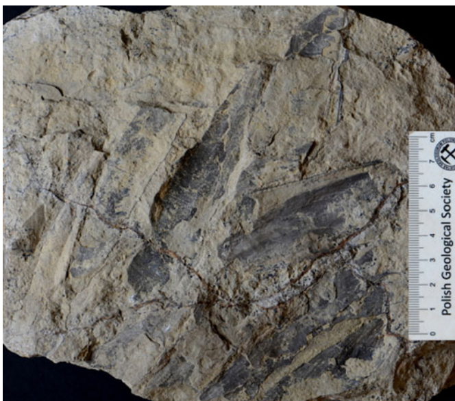
Figure 7. Aviculopinna neukirchensis shells, bedding plane group, lower carbonate cycle (Ca1), Zechstein Group, Wuchiapingian Stage, Lopingian, Permian, Nowy Kościół (Silesia), Poland.
