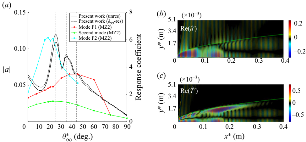
Figure 3. (a) Optimal amplitude profiles with free-stream fast acoustic waves at M_\infty = 4.5 and F = 2.2 \times 10^{-4} . (b,c) The corresponding \hat{q}^s responses (the green isocontour is \delta_{99} ). Coloured lines in panel (a) are the response coefficients from MZ2, the dashed lines are along the optimal angles from the scattering framework, and the dash-dotted line is the optimal amplitude profile with scattering sources restricted to \delta_{99} .
