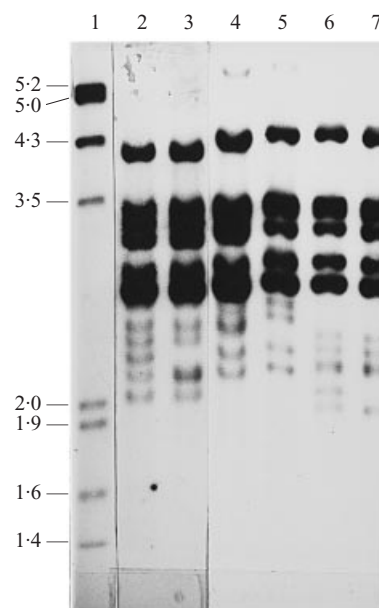
Fig. 2. HincII ribotypes of isolates of Salmonella Thompson. Lane 1, molecular size markers (kb); lanes 2 and 3, ribotypes 1 and 2; lanes 4 and 5, ribotypes 5 and 6; and lanes 6 and 7, ribotypes 3 and 4, respectively.
