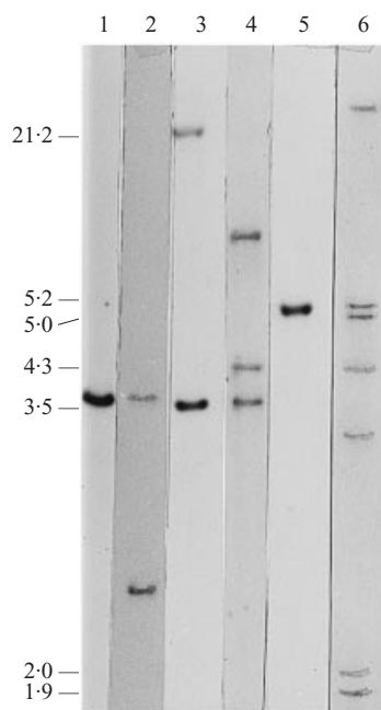
Fig. 3. PvuII -generated IS200 profiles of Salmonella Thompson. Lanes 1–5, profiles A–E, respectively; lane 6, molecular size markers (kb).
