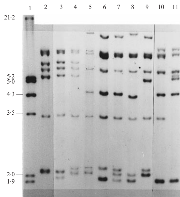
Fig. 1. PvuII ribotypes of isolates of Salmonella Thompson. Lane 1, molecular size markers (kb); lanes 2–4, ribotypes 1 and 2; lanes 4 and 5, ribotypes 5 and 6; and lanes 6 and 7, ribotypes 6 and 7; lanes 7 and 8, ribotypes 4 and 5; and lanes 9–11, ribotypes 8–10, respectively.
