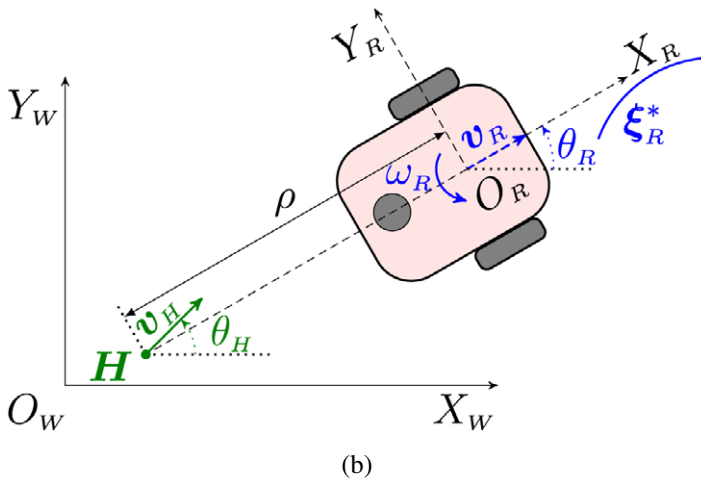
Figure 4. (a) The planned paths for the human (in green) and the robot (in blue). (b) The relative position of the human (denoted by H ) and the differential drive robot during guided walking. The (X_W, Y_W) axes represent the world (or global) coordinates, and the (X_R, Y_R) axes represent the robot (or local) coordinates.
