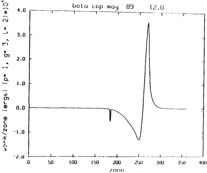
Figure 16. The work per cycle to drive oscillations is plotted versus zone number for the 400 zones of a \beta Cephei model using the opacities suggested by Rozsnyai. Peak driving at 170,000K in zone 270 is large enough to destabilize this l=2 mode. The dip at 800,000K is due to the return to the normal Iben fit.
