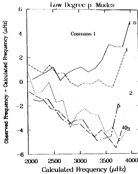
Figure 7. The observed minus the calculated low degree p-mode frequencies for the standard Cosmion model discussed in the CGR paper.
