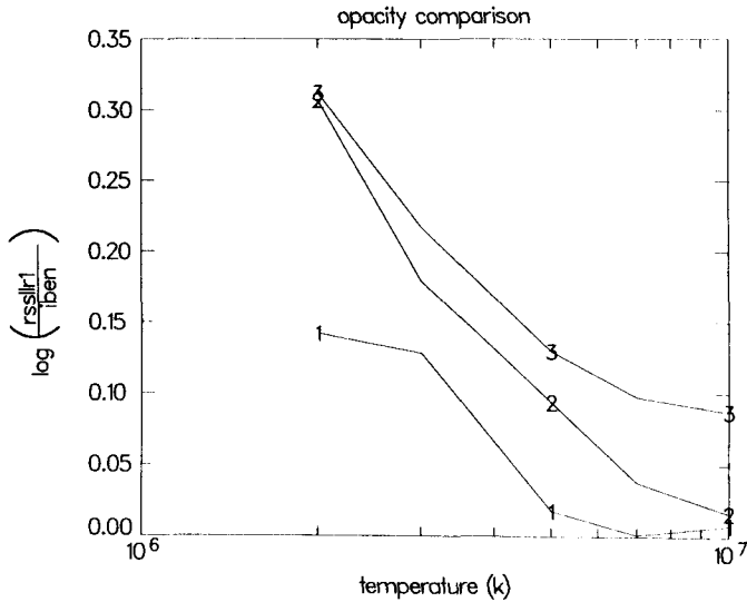
Figure 14. The logarithm of the ratio of the Ross-Aller 1 table opacities to the Iben fit procedure opacities is plotted versus temperature for densities 1 \times 10^{-1} , 1 \times 10^0 , and 1 \times 10^1 \text{ g/cm}^3 . The new Opacity Library opacities are considerably larger than those from the Iben fit originally calibrated to the Cox-Stewart opacities.
