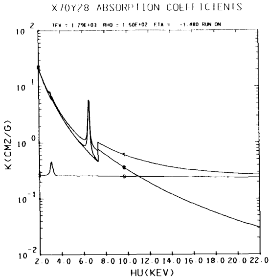
Figure 1. The monochromatic absorption coefficients for a solar mixture for the approximate solar center conditions of 15 \times 10^6 \text{K} and 150 \text{ g/cm}^3 . The iron bound-bound and bound-free transitions are seen together with the free-free absorptions from all the ions and the separately shown free electron scattering.
