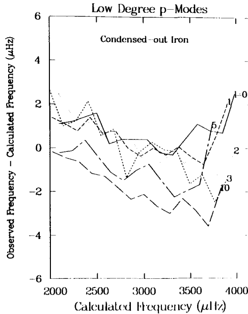
Figure 4. The observed minus the calculated low degree p-mode frequencies for the CGR condensed-out iron model.
