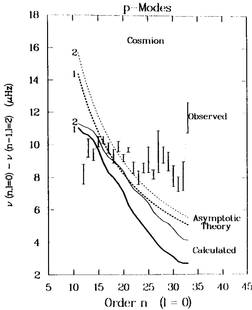
Figure 8. The \delta(n) differences between the radial and quadrupole mode frequencies is plotted versus the radial order for the two Cosmion models. The observations are given with error bars as published by Jimenez et al. (1988). Both the actually calculated eigenvalue frequency differences and the asymptotic theory variations are given.
