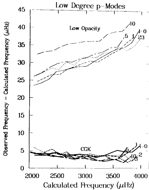
Figure 3. The observed minus the calculated low degree p-mode frequencies for the CGK and the low opacity models discussed in the CGR paper.
