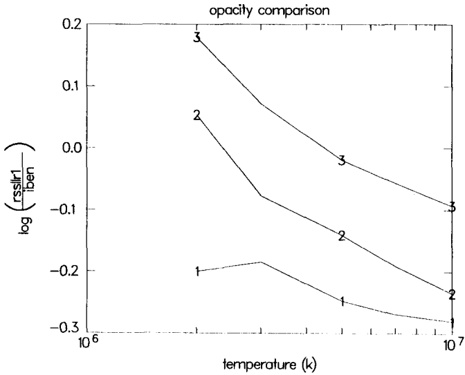
Figure 15. The logarithm of the ratio of the Ross-Aller 1 table opacities to the modified Iben fit procedure opacities is plotted versus temperature for densities 1 \times 10^{-1} , 1 \times 10^0 , and 1 \times 10^1 \text{ g/cm}^3 . At these conditions, the modified Iben fit gives opacities 15 to 20 percent larger than the Library, and these opacities give a model that has oscillation frequencies very close to those observed.
