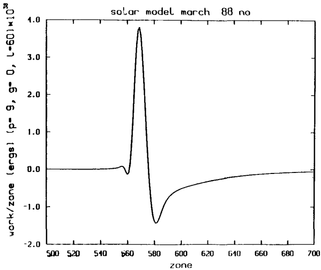
Figure 11. The work per cycle to drive oscillations is plotted versus zone number for the outer 700 zones of the 1700 mass zone CGK model using the Cox and Tabor King IVa opacity table. The peak driving at 9000K is not large enough to destabilize the mode, and this p_9 mode with l=60 decays roughly as actually observed.
