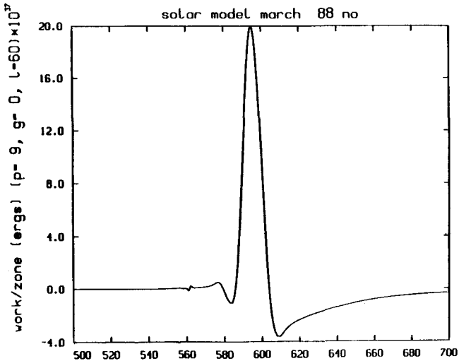
Figure 12. The work per cycle to drive oscillations is plotted versus zone number for the outer 700 zones of the 1700 mass zone CGK model using the Opacity Library Ross-Aller 1 opacity table to calibrate the Stellingwerf fit. The peak driving at 9000K is large enough to destabilize this p_9 mode with l=60 .
