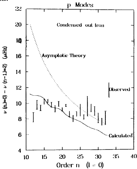
Figure 6. The \delta(n) differences between the radial and quadrupole mode frequencies are plotted versus the radial order for the condensed-out iron model. Observations are given with error bars (Jimenez et al., 1988). Both the calculated eigenvalue frequency differences and the asymptotic theory variations are given.
