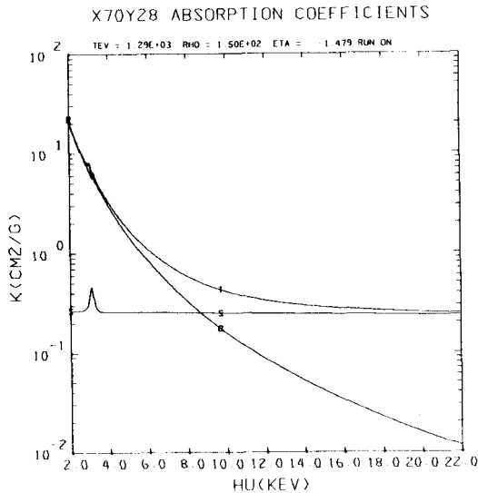
Figure 2. The monochromatic absorption coefficients for a solar mixture without iron for the approximate solar center conditions of 15 \times 10^6 \text{K} and 150 \text{ g/cm}^3 . The iron line and bound-free edge are now absent, and the opacity is reduced from 1.18 \text{ cm}^2/\text{g} to 0.92 \text{ cm}^2/\text{g} .
