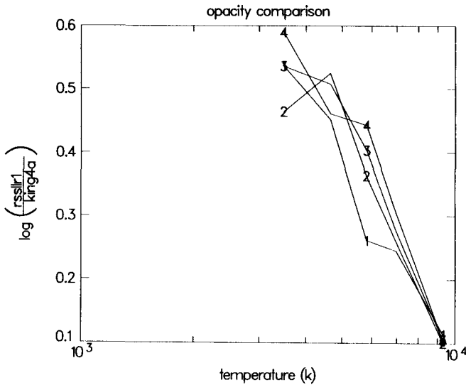
Figure 9. The logarithm of the ratio of the Ross-Aller 1 table opacities to the King IVa table opacities is plotted versus temperature for densities 3 \times 10^{-8} , 1 \times 10^{-7} , 3 \times 10^{-7} , and 1 \times 10^{-6} \text{ g/cm}^3 . At the solar photosphere, the new Opacity Library opacities are twice that from the Cox and Tabor tables.
