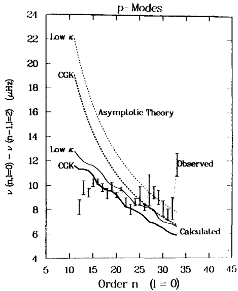
Figure 5. The \delta(n) differences between the radial and quadrupole mode frequencies is plotted versus the radial order for the CGK and the low opacity models. The observations are given with error bars as published by Jimenez et al. (1988). Both the actually calculated eigenvalue frequency differences and the asymptotic theory variations are given.
