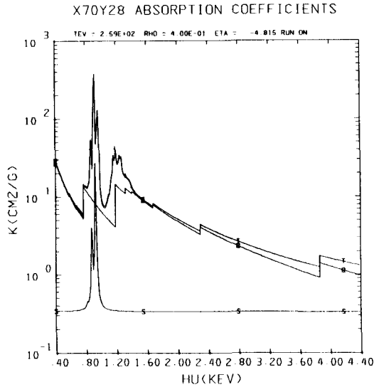
Figure 13. The monochromatic absorption coefficients for a solar mixture for the approximate solar conditions below the convection zone of 3 \times 10^6 K and 0.4 \text{ g/cm}^3 . Absorption K edges of oxygen, neon, magnesium, aluminum, silicon, and argon can be seen. Also at 1.4 kilovolt photon energy weak closely spaced L edges of iron are visible.
