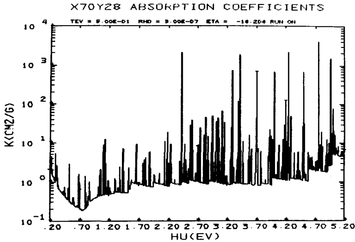
Figure 10. The monochromatic absorption coefficients for a solar mixture for the approximate solar photosphere conditions of 5800\text{K} and 3 \times 10^{-7} \text{ g/cm}^3 . On top of the dominant negative hydrogen ion absorption one can see the myriad of iron lines coming from transitions from the M shell to higher levels.
