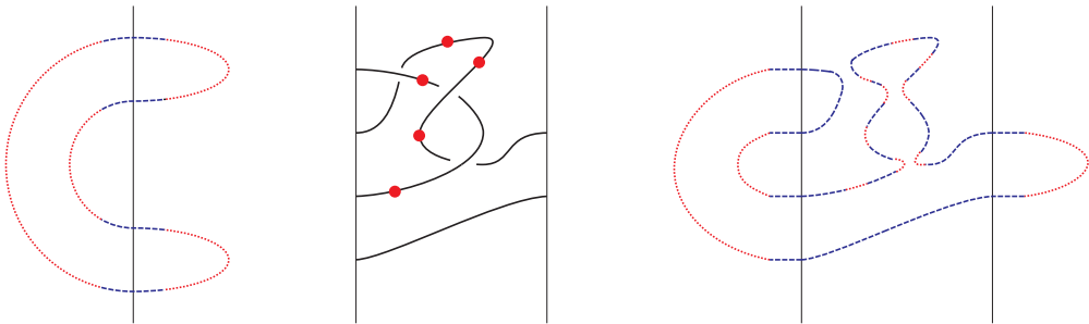
Figure 3.1. Active arcs and flat tangles. Left: a\bar{b} for two crossingless matchings a, b \in \mathbb{B}_2 and the decomposition of a\bar{b} into active (dotted) and inactive (dashed) arcs. Center: a poxed (4,2) -tangle T . Right: aT_v\bar{b} where v = (1,0,0) and a is the same crossingless matching as on the left.
