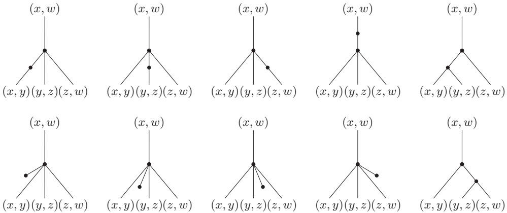
Figure 2.1. Some of the multimorphisms in \text{Hom}((x,y),(y,z),(z,w);(x,w)) from Example 2.7. The edges are labelled by the objects and the internal vertices are labelled by multimorphisms in the original multicategory (i.e., basic multimorphisms). Edges ending in a node are stumps. The original multicategory being the shape multicategory of a set, the vertex labels and the internal edge labels are forced and are not shown.
