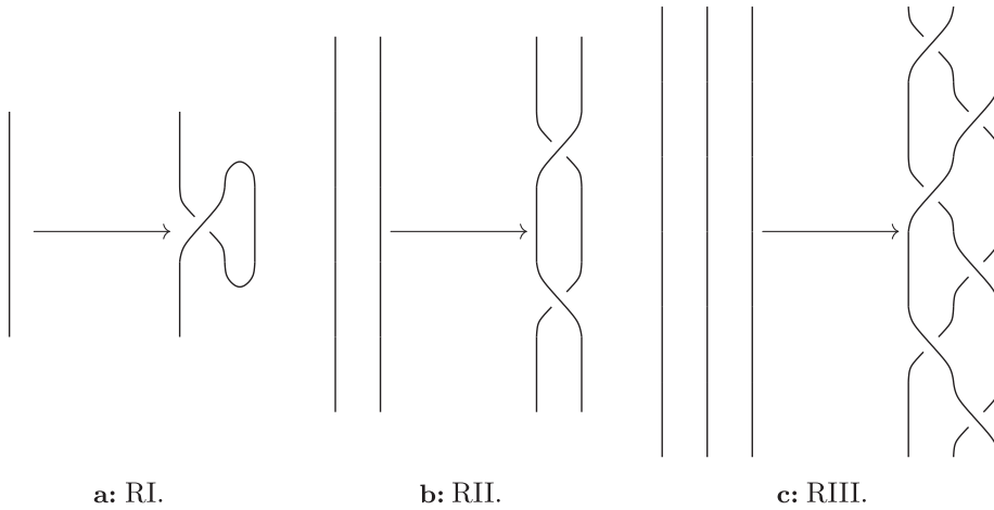
Figure 3.3. Reidemeister moves. The orientations of the strands are arbitrary. This figure originally appeared in [41].
