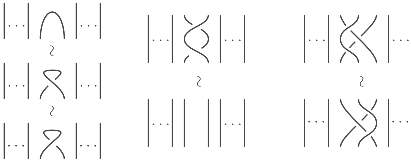
Figure 3.4. Local Reidemeister moves. Khovanov’s invariance proof shows that the bimodules before and after each Reidemeister move are quasi-isomorphic and in fact there is an essentially unique, up to sign, quasi-isomorphism between them.
