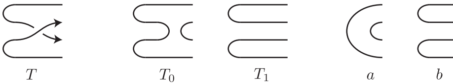
Figure 7.1. Where have all the ladybugs gone? Left: a tangle T . Center: the resolutions T_0 and T_1 of T . Right: the crossingless matchings a and b .
