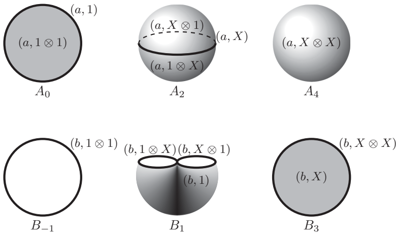
Figure 7.2. Some mapping cones. The space \mathcal{X}(T)(a) is the wedge sum of the spaces A_0 , A_2 and A_4 , and \mathcal{X}(T)(b) is the wedge sum of the spaces B_{-1} , B_1 and B_3 (the subscripts denote the quantum gradings). A cellular decomposition is shown with the cells labelled by the corresponding Khovanov generators. The space A_2 is built from one 1-cell labelled (a, X) and two 2-cells labelled (a, 1 \otimes X) and (a, X \otimes 1) . The space B_1 has two 1-cells labelled (b, 1 \otimes X) and (b, X \otimes 1) and one 2-cell labelled (b, 1) .
