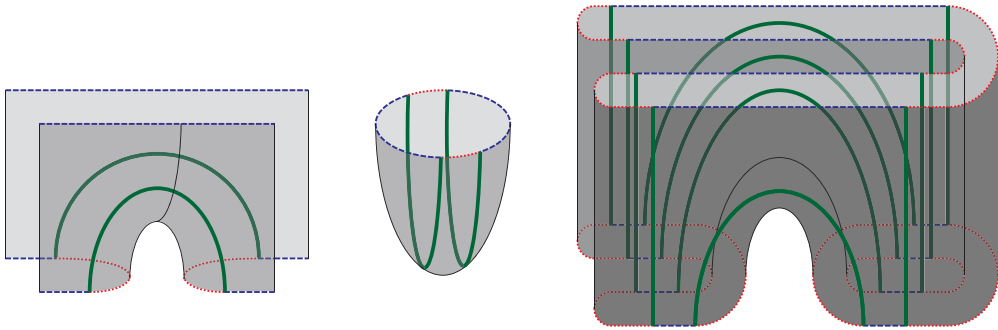
Figure 3.2. Basic divided cobordisms. Left: a saddle. Center: a cup. Curves \Gamma are thick, arcs in I \cup I' are dashed and arcs in A \cup A' are dotted. Together with product cobordisms, these are the local pieces that the divided cobordisms of interest are built from. Right: the divided cobordism associated to a product on the Khovanov arc algebra.
