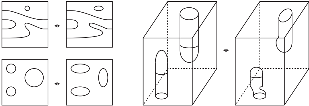
Figure 2.2. The actions of \text{Diff}^1 and \text{Diff}^2 . Left: two flat (4,2) -tangles related by the action of \text{Diff}^1 \times \text{Id} and two flat (0,0) -tangles related by the action of \text{Diff}^1 \times \text{Id} . Right: two flat (0,0) -tangle cobordisms related by the action of \text{Diff}^2 \times \text{Id} .
