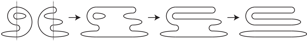
Figure 2.3. Flat tangles and the multiplication on \mathcal{H}^n .
