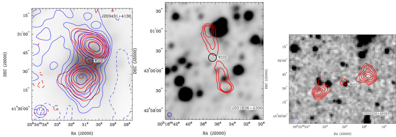
Figure C2. GMRT contours at 610 MHz (red) and 325 MHz (blue) overlaid on WISE/2MASS infrared images. The contour levels at 325 MHz are the same shown in Figures A1-A6. The contour levels at 610 MHz are: #35-J203431+413037: -2.5, 2.5, 9, 15, 21, 35, and 55 , in units of \sigma (= 0.12 \text{ mJy beam}^{-1}) . #40-J201836+430018: -2.5, 2.5, 10, and 20 , in units of \sigma (= 0.5 \text{ mJy beam}^{-1}) . #42-J203431+413035: -2.5, 2.5, 5, 9, 15, 21, 35, 55, and 85 , in units of \sigma (= 0.15 \text{ mJy beam}^{-1}) . The synthesised beams are shown at the bottom left corner of each image.
