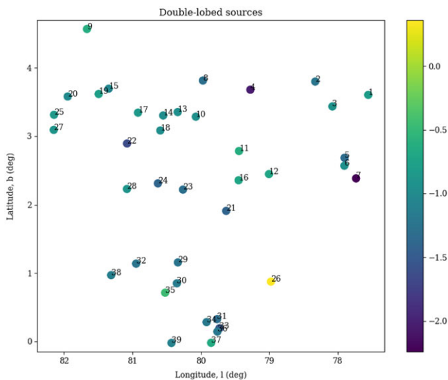
Figure 2. Layout of the observed double-lobed sources in Galactic coordinates, with their spectral indices represented with colours, according to the scale at the right.
