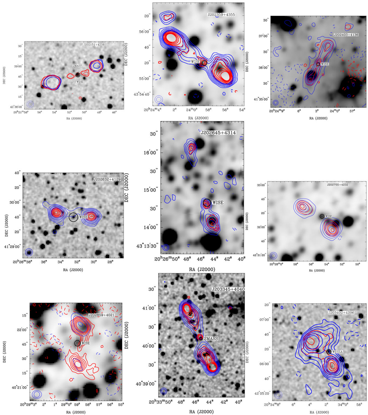
Figure C1. GMRT contours at 610 MHz (red) and 325 MHz (blue) overlaid on WISE (W1-band)/2MASS (3.4 \mu\text{m} ) infrared images. The contour levels at 325 MHz are the same shown in Figures A1-A6. The contour levels at 610 MHz are: #10-J202151+423847: -2.5, 2.5, 3, and 5, in units of \sigma ( = 0.13 \text{ mJy beam}^{-1} ). #15-J202352+435525: -2.5, 2.5, 5, 9, 15, 21, and 27, in units of \sigma ( = 0.1 \text{ mJy beam}^{-1} ). #16-J202403+413611: -2.5, 2.5, 5, and 15, in units of \sigma ( = 0.15 \text{ mJy beam}^{-1} ). #21-J202632+412942: -2.5, 2.5, 5, 10, 15, 25, and 35, in units of \sigma ( = 0.1 \text{ mJy beam}^{-1} ). #22-J202645+431435: -2.5, 2.5, 5, 9, and 15, in units of \sigma ( = 0.1 \text{ mJy beam}^{-1} ). #24-J202755+423215: -2.5, 2.5, 30, 50, and 130, in units of \sigma ( = 0.1 \text{ mJy beam}^{-1} ). #26-J202859+402141: -2.5, 2.5, 9, 15, 21, and 27, in units of \sigma ( = 0.1 \text{ mJy beam}^{-1} ). #31-J203345+404015: -2.5, 2.5, 9, 15, 21, and 27, in units of \sigma ( = 0.2 \text{ mJy beam}^{-1} ). #32-J203402+420615: -2.5, 2.5, 9, 15, 21, and 27, in units of \sigma ( = 0.1 \text{ mJy beam}^{-1} ). The synthesised beams are shown at the bottom left corner of each image.
