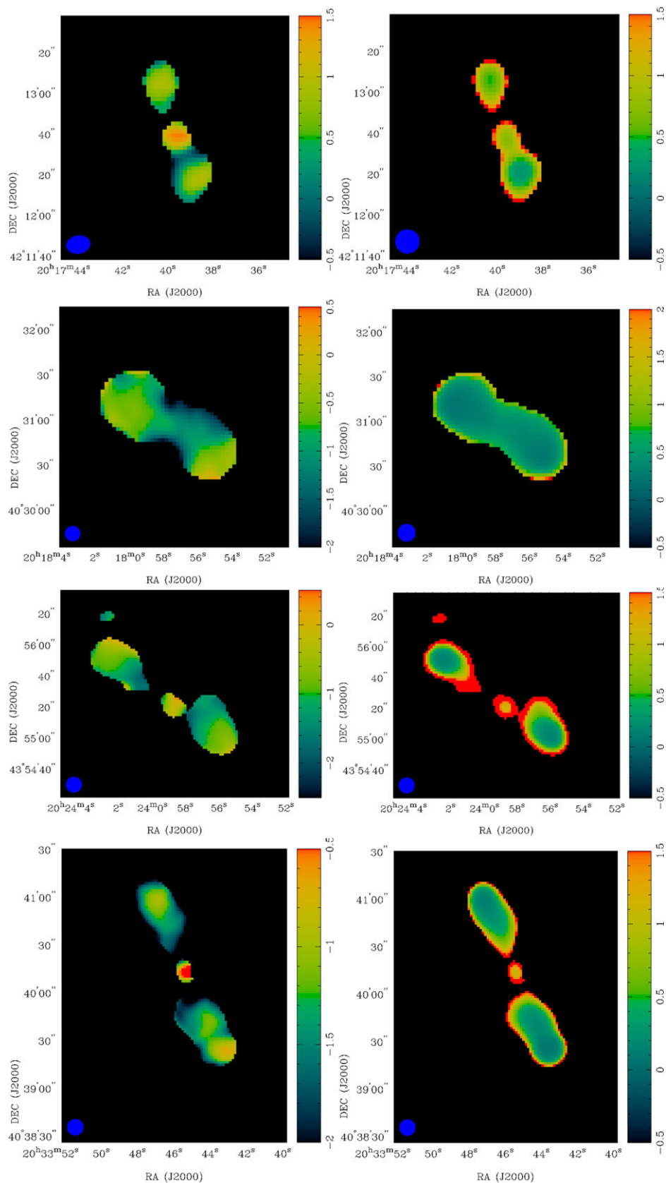
Figure B1. Spectral index (left) and error maps (right) of J201739+421252 (#4, first row), J201758+403100 (#5, second row), J202359+435525 (#15, third row), and J203345+404015 (#31, fourth row) sources. The synthesised beam is shown at the bottom left corner of each image.
