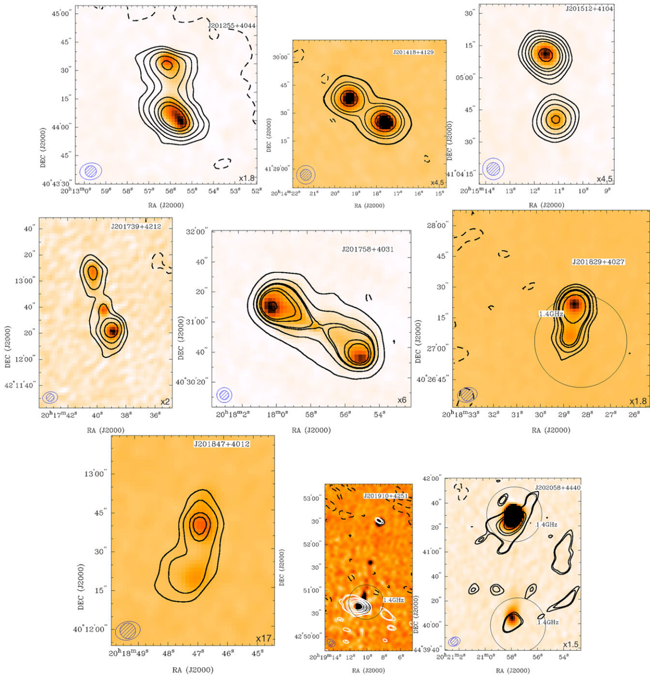
Figure A1. GMRT images of the double-lobed sources at 610 MHz (colour scale) and 325 MHz (contours). The contour levels and colour scale interval for each source are as follows: #1-J201255+4044: -2.5, 2.5, 3, 15, 27, 60, and 90, in units of \sigma ( =0.18 \text{ mJy beam}^{-1} ); [1.6, 20] \text{mJy beam}^{-1} . #2-J201418+4129: -2.5, 2.5, 3, 15, 27, 60, and 90, in units of \sigma ( =0.45 \text{ mJy beam}^{-1} ); [3, 13] \text{mJy beam}^{-1} . #3-J201512+4104: -2.5, 2.5, 5, 9, 15, 21, and 41, in units of \sigma ( =0.45 \text{ mJy beam}^{-1} ); [4, 11] \text{mJy beam}^{-1} . #4-J201739+4212: -2.5, 2.5, 5, 9, 21, and 27, in units of \sigma ( =0.2 \text{ mJy beam}^{-1} ); [0.4, 4] \text{mJy beam}^{-1} . #5-J201758+4031: -2.5, 2.5, 15, 27, 30, 45, 55, and 100, in units of \sigma ( =0.6 \text{ mJy beam}^{-1} ); [0.6, 17] \text{mJy beam}^{-1} . #6-J201829+4027: -2.5, 2.5, 3, 15, 27, 60, and 90, in units of \sigma ( =0.18 \text{ mJy beam}^{-1} ); [6, 21] \text{mJy beam}^{-1} . #7-J201847+4012: -2.5, 2.5, 5, 9, 11, and 21, in units of \sigma ( =1.7 \text{ mJy beam}^{-1} ); [6, 21] \text{mJy beam}^{-1} . #8-J201910+4251: -2.5, 2.5, 3, 6, 9, 15, 21, and 30, in units of \sigma ( =0.7 \text{ mJy beam}^{-1} ); [0.7, 9] \text{mJy beam}^{-1} . #9-J202058+4440: -2.5, 2.5, 3, 15, 27, 60, and 90, in units of \sigma ( =0.15 \text{ mJy beam}^{-1} ); [0.7, 9] \text{mJy beam}^{-1} . The synthesised beams are shown at the bottom left corner of each image. NVSS detections are marked with a 45'' diameter circle and labelled as '1.4 GHz'. For the x factor of the bottom right corner, see text.
