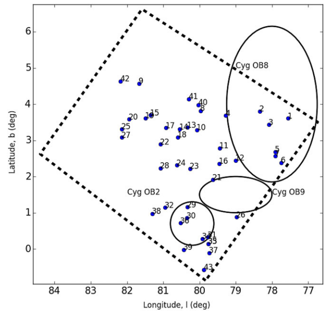
Figure 1. Observed area of the Cygnus constellation marked with a black dashed contour box, over the identified stellar associations Cygnus OB2 and Cygnus OB8 as well as Cygnus OB9. The blue dots are the double-lobed sources presented in this paper, with ID numbers as in Table 1.
