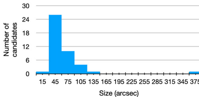
Figure 4. Distribution of sizes of the 43 double-lobed candidates. The extension of the sources ranged from \sim 25 arcsec up to \sim 375 arcsec ( \sim 7 arcmins).
