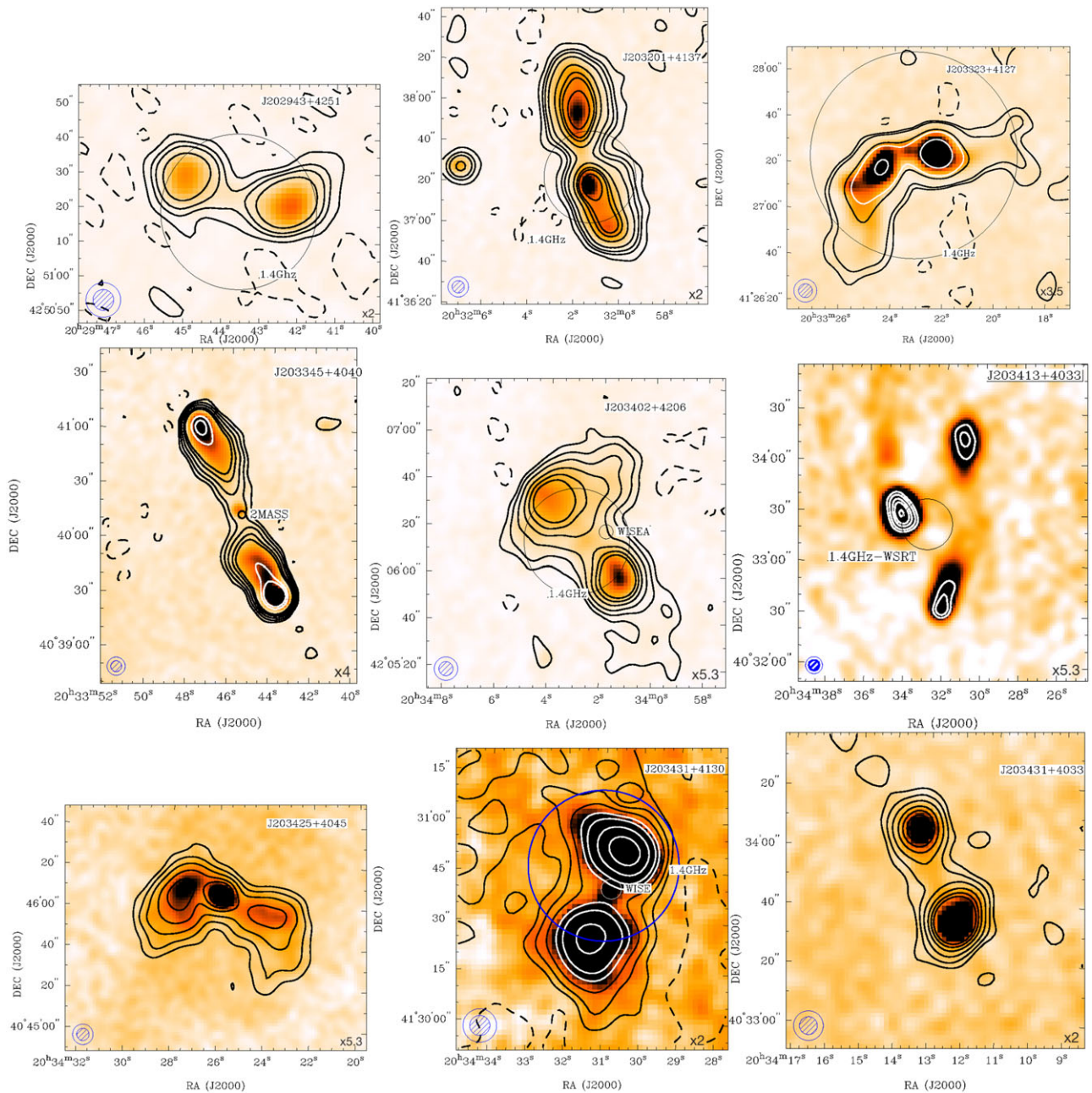
Figure A4. GMRT images of the double-lobed sources at 610 MHz (colour scale) and 325 MHz (contours). The contour levels and colour scale interval for each source are as follows: #28-J202943+425122: -2.5, 2.5, 9, 15, 27 in units of \sigma (= 0.2 \text{ mJy beam}^{-1}) ; [0.4, 1] \text{mJy beam}^{-1} . #29-J203201+413730: -2.5, 2.5, 9, 15, 27, 57, 87, 107, and 150, in units of \sigma (= 0.2 \text{ mJy beam}^{-1}) ; [0.4, 1] \text{mJy beam}^{-1} . #30-J203323+412720: -2.5, 2.5, 5, 27, 40, and 100, in units of \sigma (= 0.35 \text{ mJy beam}^{-1}) ; [0.6, 5] \text{mJy beam}^{-1} . #31-J203345+404015: -2.5, 2.5, 5, 9, 15, 21, 55, and 75, in units of \sigma (= 0.4 \text{ mJy beam}^{-1}) ; [0.5, 5] \text{mJy beam}^{-1} . #32-J203402+420615: -2.5, 2.5, 5, 9, 15, 21, and 27, in units of \sigma (= 0.53 \text{ mJy beam}^{-1}) ; [0.4, 10] \text{mJy beam}^{-1} . #33-J203413+403349: -2.5, 2.5, 5, 9, 15, 21, and 27, in units of \sigma (= 0.53 \text{ mJy beam}^{-1}) ; [0.4, 10] \text{mJy beam}^{-1} . #34-J203425+404605: -2.5, 2.5, 5, 9, 15, 21, and 27, in units of \sigma (= 0.53 \text{ mJy beam}^{-1}) ; [0.3, 2.8] \text{mJy beam}^{-1} . #35-J203431+413037: -2.5, 2.5, 5, 9, 15, 21, 35, and 55, in units of \sigma (= 0.2 \text{ mJy beam}^{-1}) ; [0.4, 14] \text{mJy beam}^{-1} . #36-J203431+403332: -2.5, 2.5, 5, 9, 15, 21, and 27, in units of \sigma (= 0.53 \text{ mJy beam}^{-1}) ; [0.2, 0.7] \text{mJy beam}^{-1} . The synthesised beams are shown at the bottom left corner of each image. NVSS and WSRT beams detection are marked with a circles and labelled as '1.4 GHz' and '1.4GHz-WSRT'. WISE and 2MASS position errors are marked with circles and labelled as well. For the x factor of the bottom right corner, see text.
