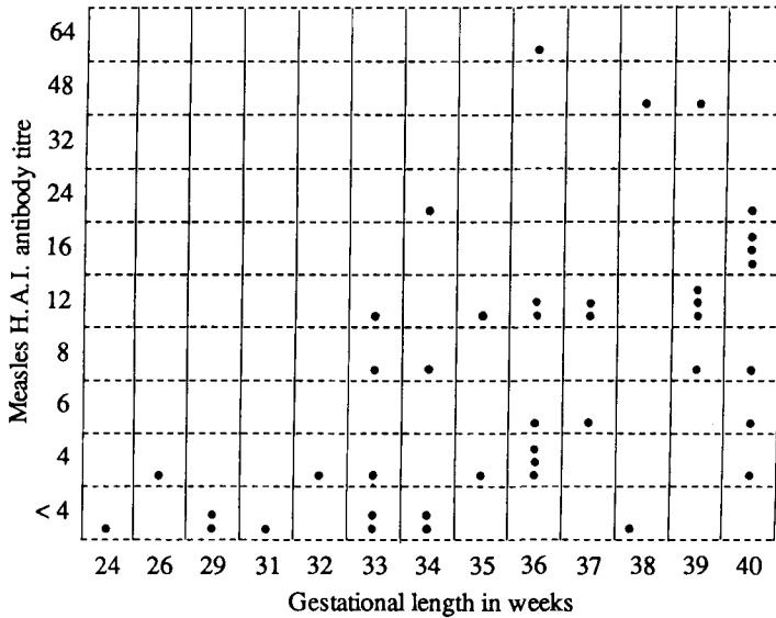
Fig. 2. HI titres for neonates of different gestational length.
