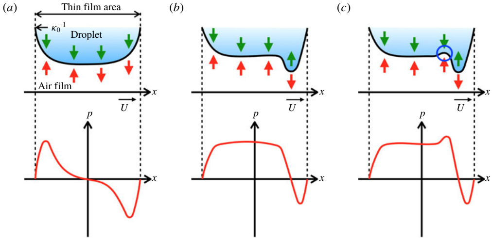
FIGURE 13. (Colour online) Schematic views of the process of air film shape formation along with the lubrication pressure and surface tension pressure in two dimensions. Upper: the gas–liquid surface shape shown as a black line, direction of lubrication pressure shown as red arrows and direction of surface tension pressure shown as green arrows. Lower: lubrication pressure. (a) Lubrication pressure has positive pressure upstream and negative pressure downstream while the surface tension pressure has positive pressure over the whole range. (b) The gas–liquid surface has a plateau in the centre of the droplet and a minimum thickness downstream. (c) A high lubrication pressure due to the steep surface region (wedge effect) arises by decreasing the air film thickness in the downstream side, and the pressure increases at the blue circle. As a result, dimple formation is generated.
