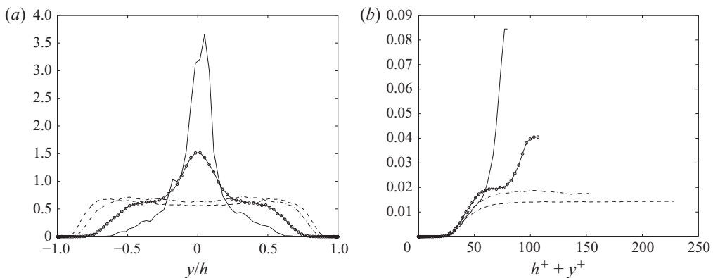
FIGURE 7. Probability density function of low speed streak positions computed considering the instantaneous location of the minimum value of wall skin friction: (a) in outer units and (b) in inner units (the origin has been translated to the corner). —, Re_b = 1100 ; —●—, Re_b = 1500 ; - · - · - , Re_b = 2200 ; - - - - , Re_b = 3500 .
