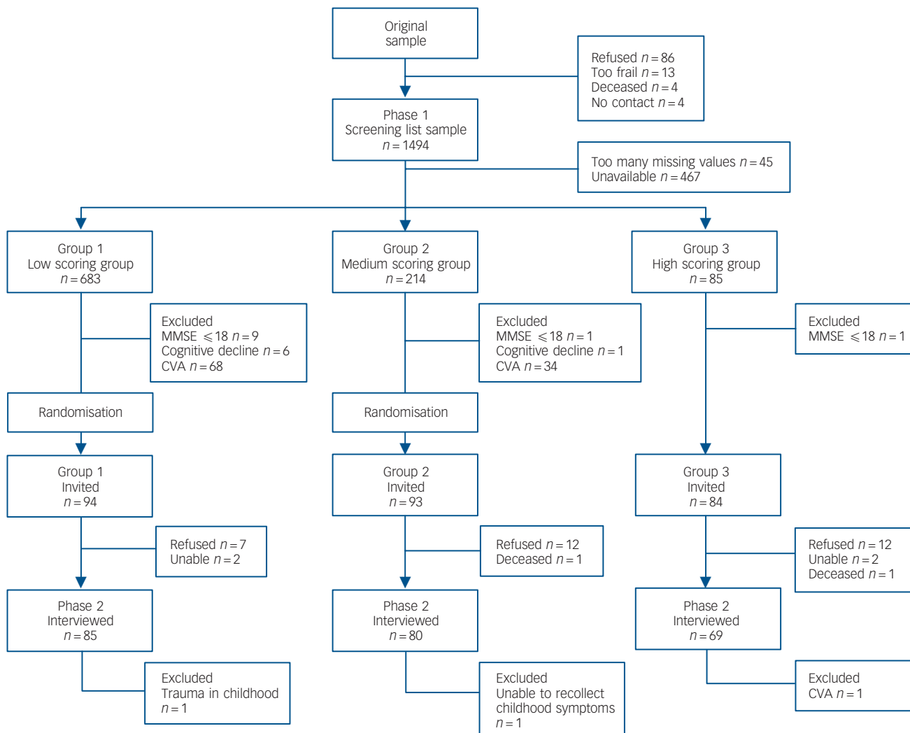
Fig. 1 Flowchart of screening and diagnostic interview phases. CVA, cerebrovascular accident; MMSE, Mini-Mental State Examination.
