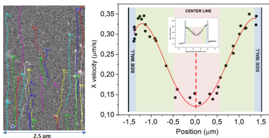
Figure 2. Flow in nanochannel observed by STEM, and tracked by subtracting the first image to remove background. The channels have an inwards deflection and hence a thinner liquid layer at the center of the channel as indicated by the insert showing a STEM signal profile across the channel. The measured flow velocities match a parabolic flow profile with lower flow velocities at the center and also lower near the channel walls.
