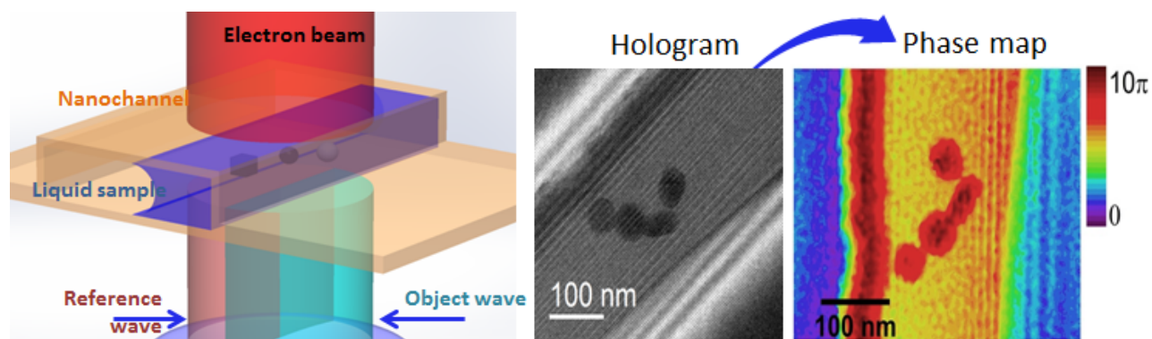
Figure 1. Electron holographic imaging of liquid samples in a suspended nanochannel gives a holographic image that can provide a phase map of the liquid sample.
