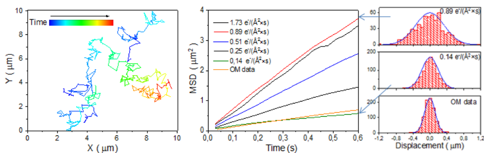
Figure 3. Brownian motion of a freely moving gold nanoparticle in a liquid cell. Mean square displacement and step length histogram indicate Brownian motion with a diffusion coefficient depending on the beam current density.
