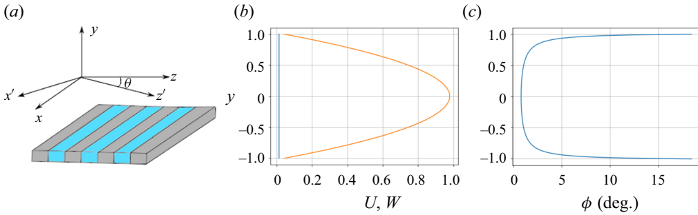
Figure 1. (a) Sketch of the SH surface covered with riblets oriented at an angle \theta with respect to the streamwise direction. (b) Streamwise (orange) and spanwise (blue) velocity components of the base flow for \lambda_{\parallel} = 0.03 and \theta = 45^\circ . (c) Angle between the bulk velocity and the pressure gradient.
